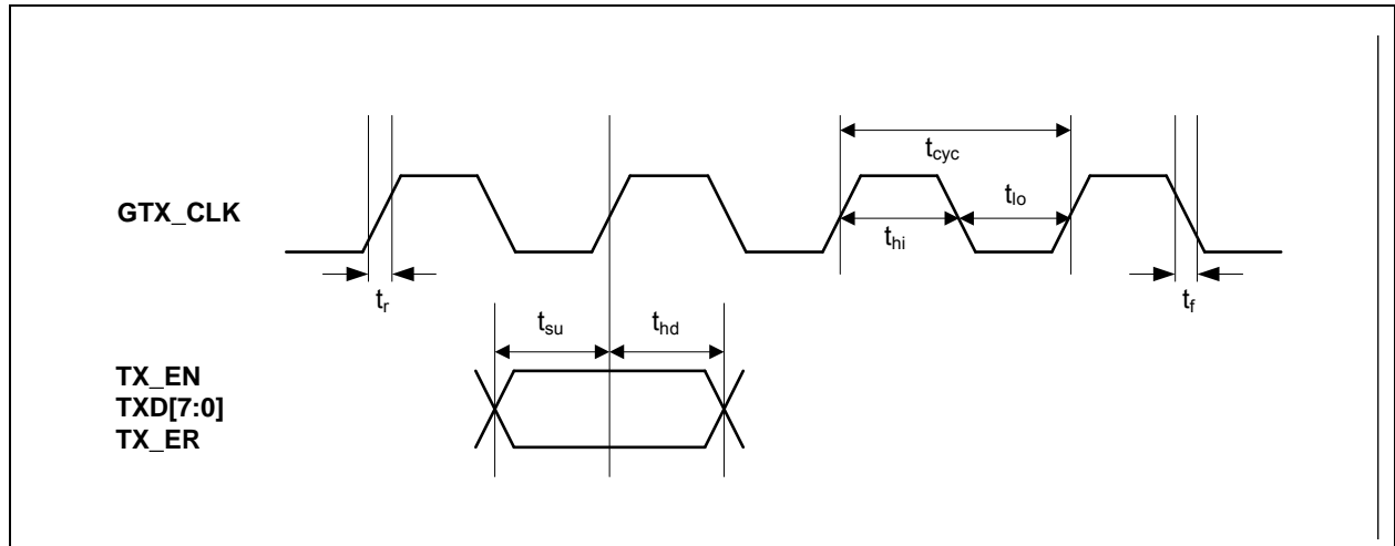
FIGURE 6-1: GMII TRANSMIT TIMING – DATA INPUT TO PHY
