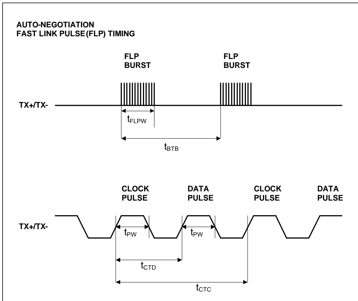
FIGURE 6-5: AUTO-NEGOTIATION FAST LINK PULSE (FLP) TIMING
