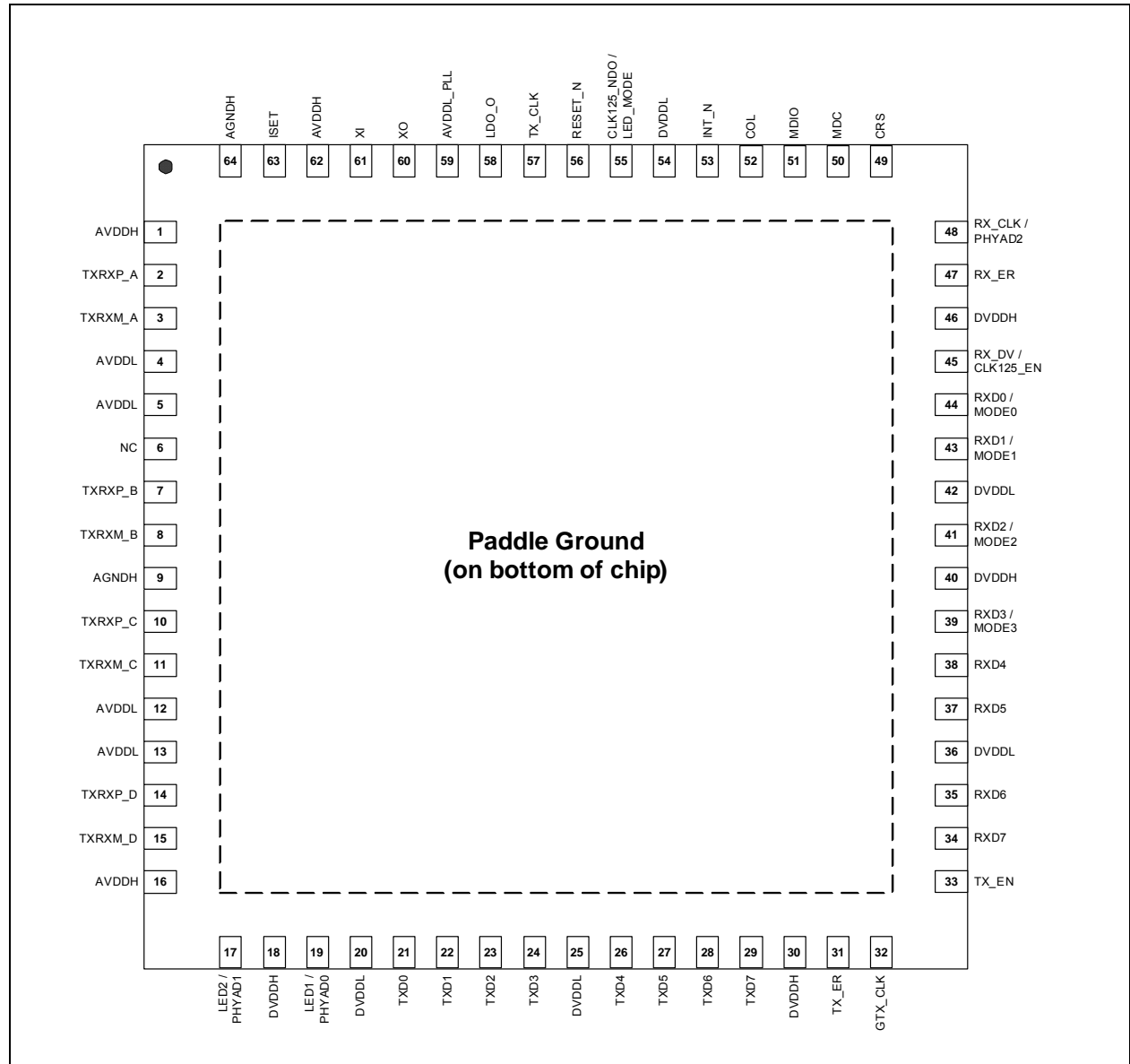
FIGURE 2-1: 64-PIN QFN (TOP VIEW)
