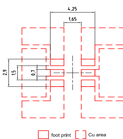
Component Location on Pad
