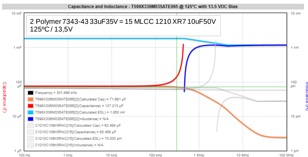
Figure 9. Capacitance in frequency at 125°C and 13,5V – K-SIM
