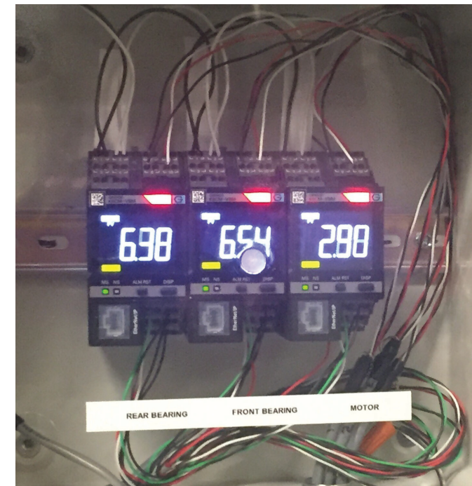
The K6CM Motor Condition Monitoring Device from Omron
