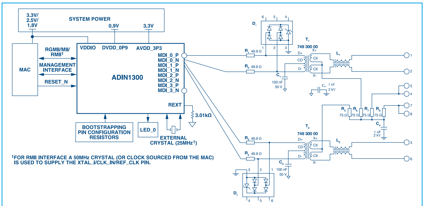
Figure 5 - Simplified Typical Application Block Diagram.
