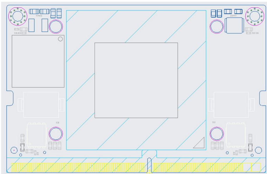
Figure 1-5. Jetson Orin Nano 4GB Topside View
