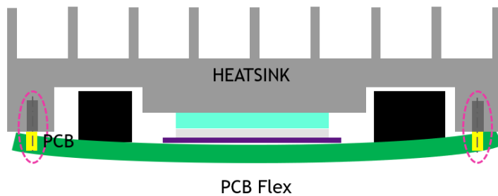
Figure 4-4. PCB Flex
