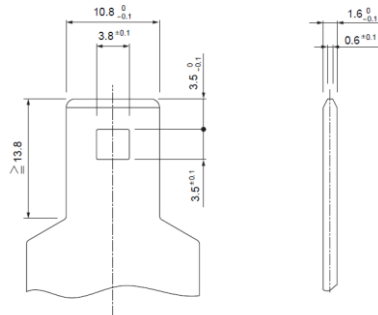
Recommended bracket layout
