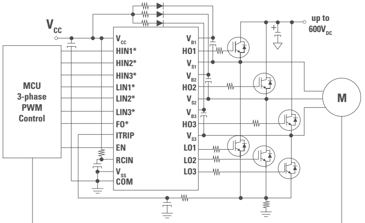
LF2136 Application Circuit
