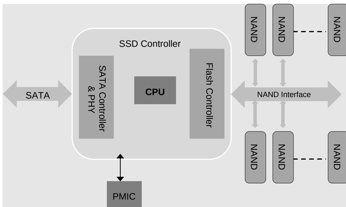
Figure 1 – Block Diagram
