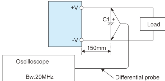
Fig.1.1 Measuring method for Ripple and Ripple Noise
