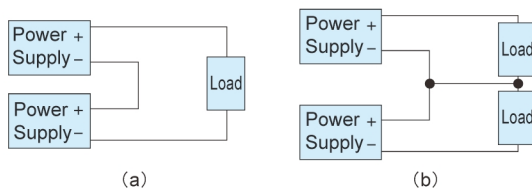
Fig.2.1 Examples of connecting in series operation
