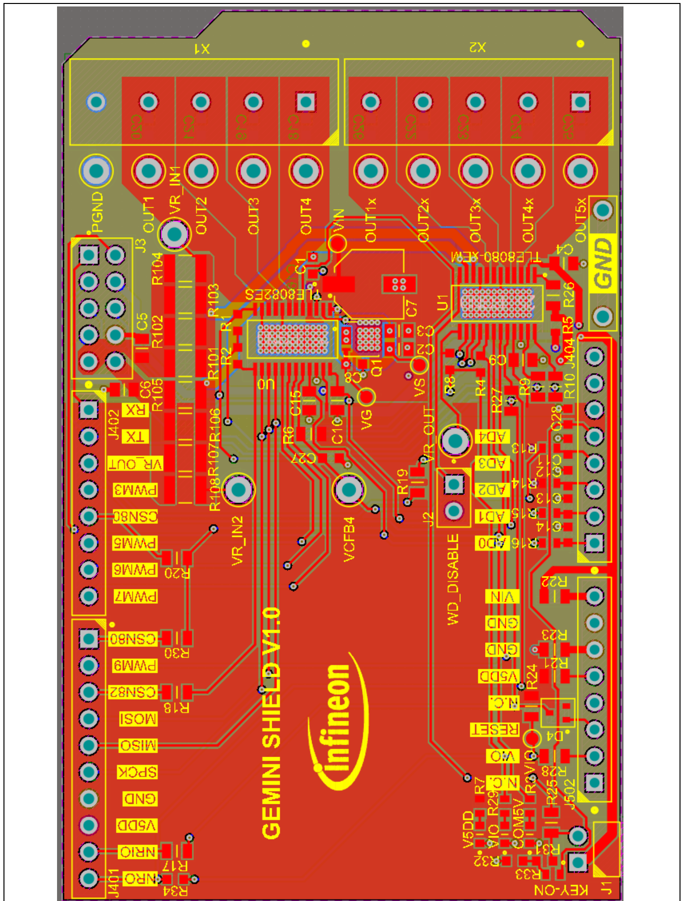
Figure 11 Layout Evaluation-PCB
