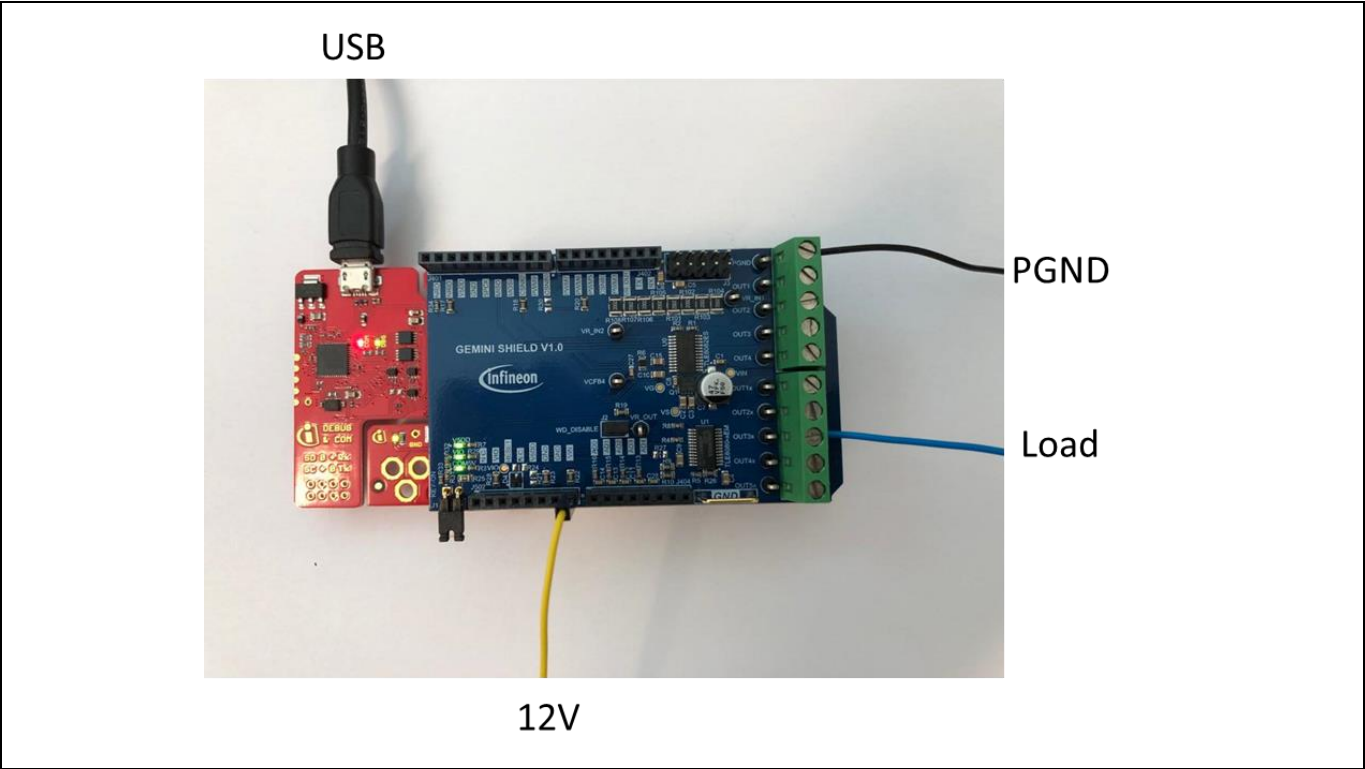
Figure 2 Illustration of XMC Hardware setup
