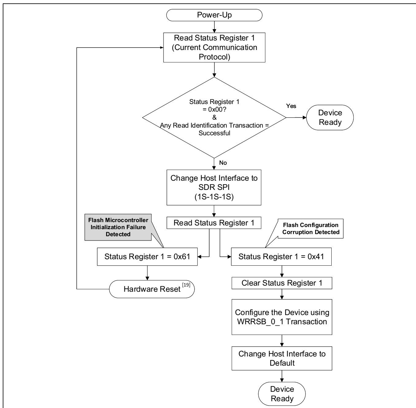
Figure 53 Host polling sequence for microcontroller initialization failure detection
