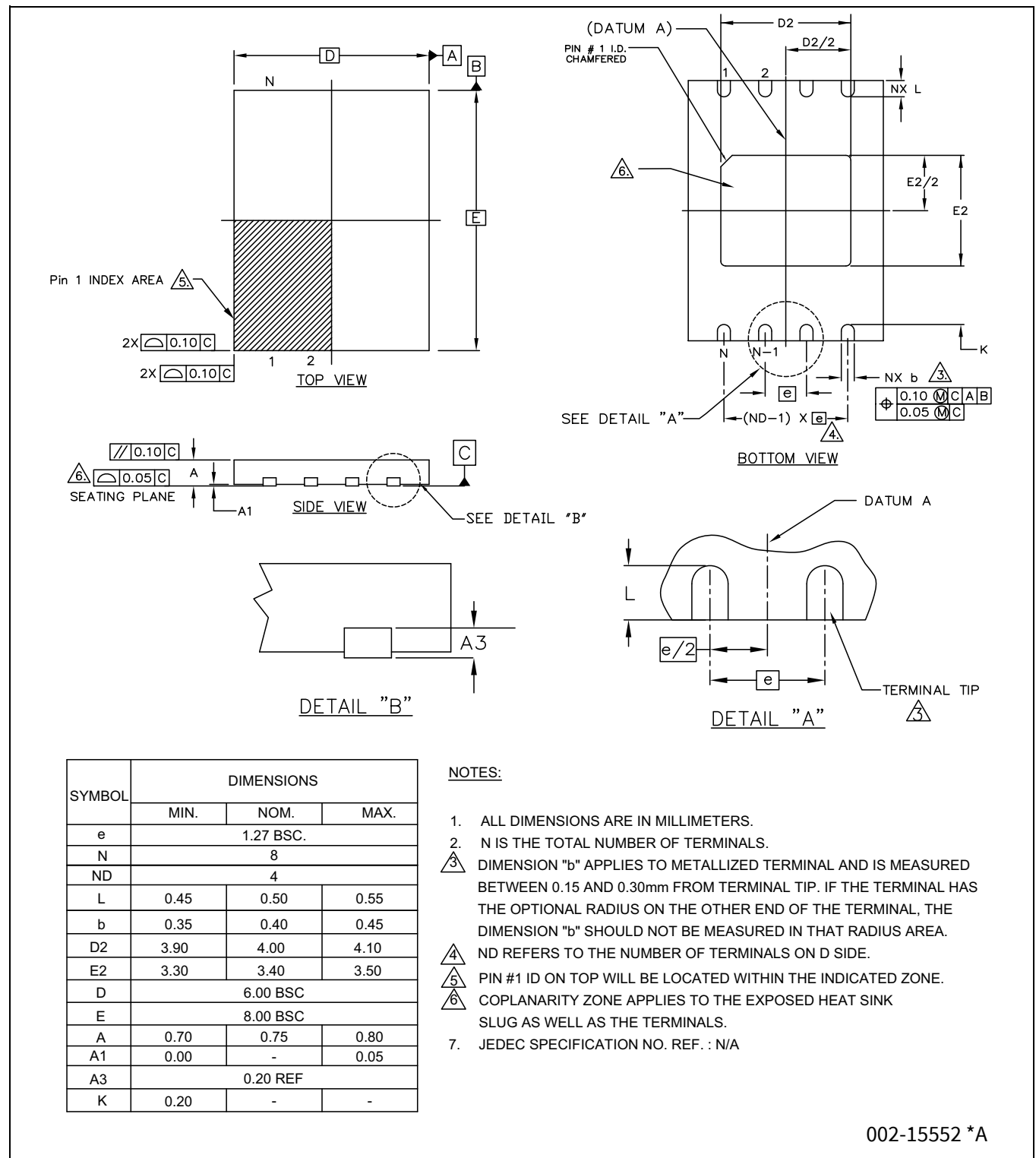
Figure 88 8-lead DFN (6.0 × 8.0 × 0.8 mm) 4.0 × 3.4 mm E-Pad (Sawn) package outline, 002-15552
