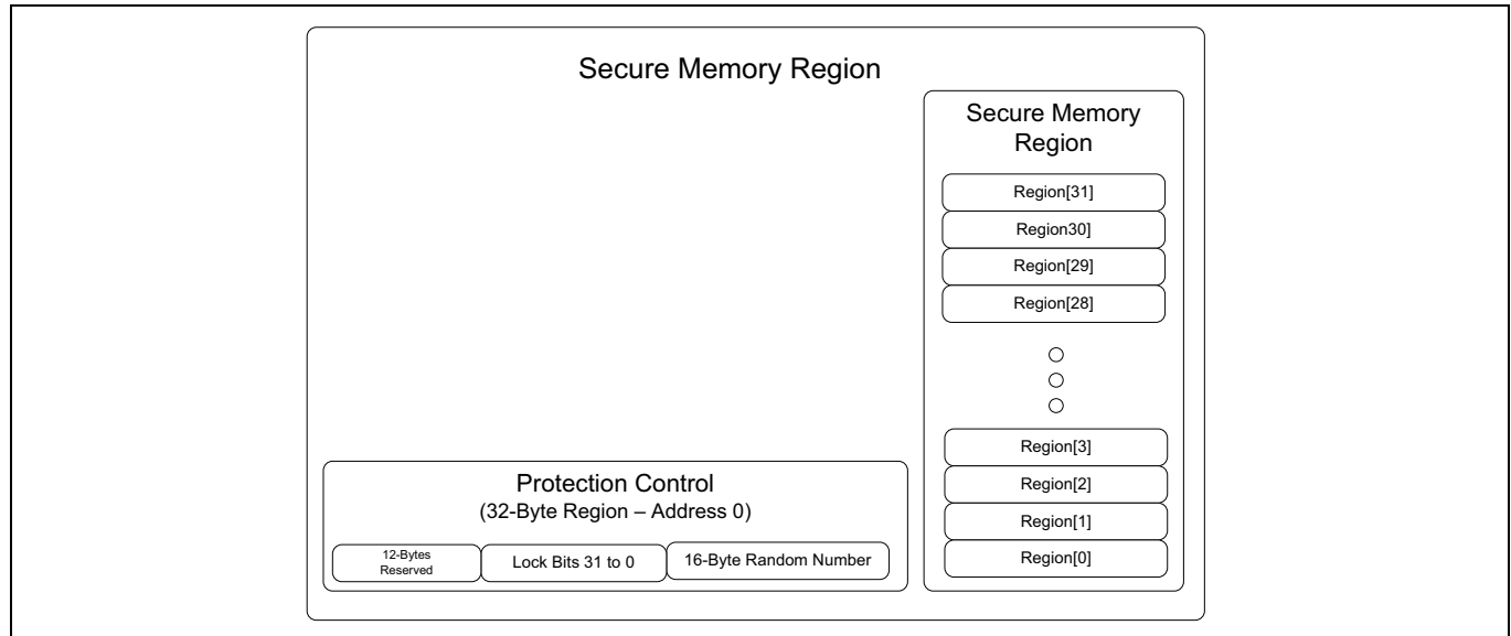
Figure 52 OTP protection (nonvolatile)
