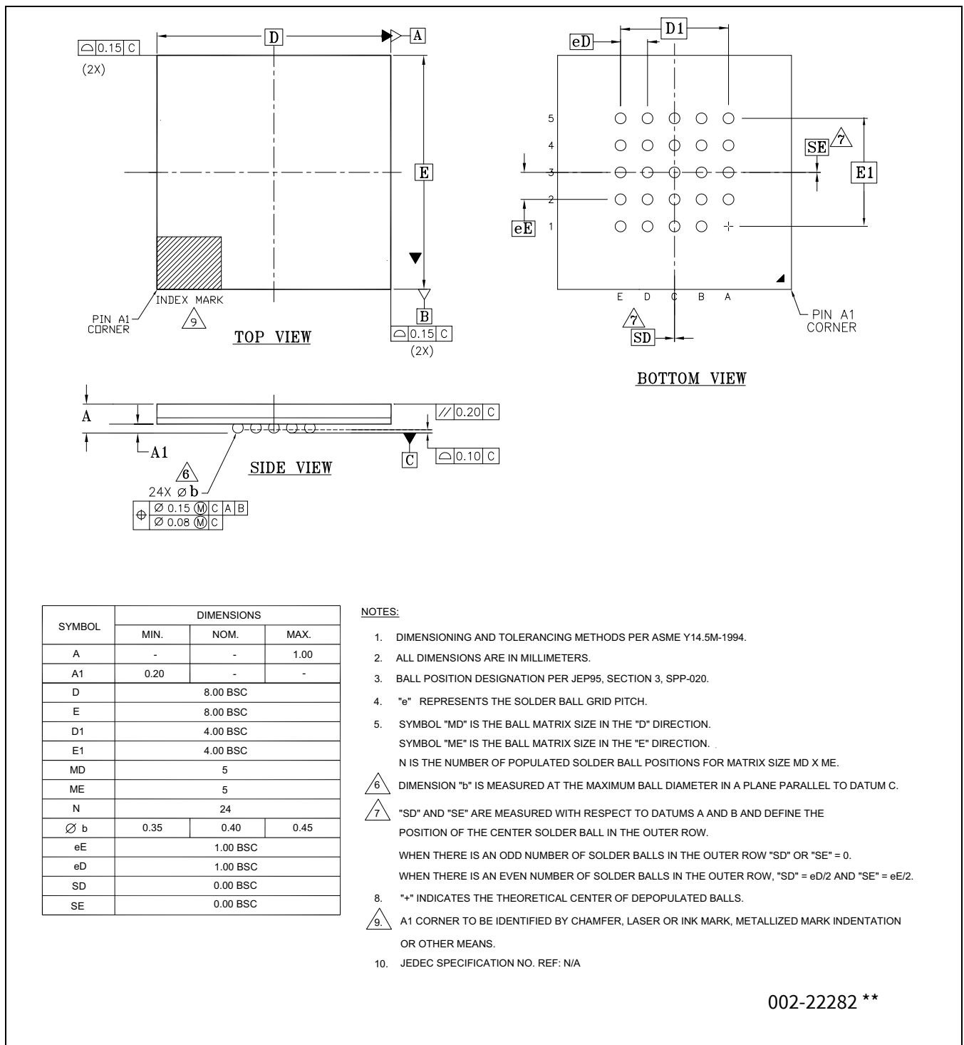
Figure 86 24-ball BGA (8.0 x 8.0 x 1.0 mm) package outline, 002-22282
