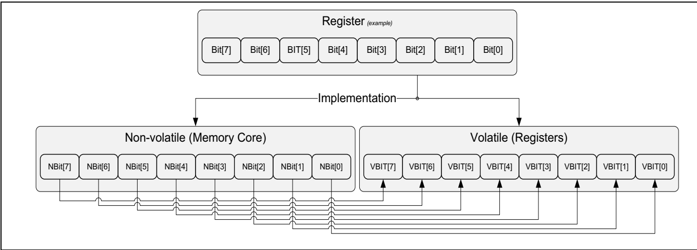
Figure 68 Register structure
