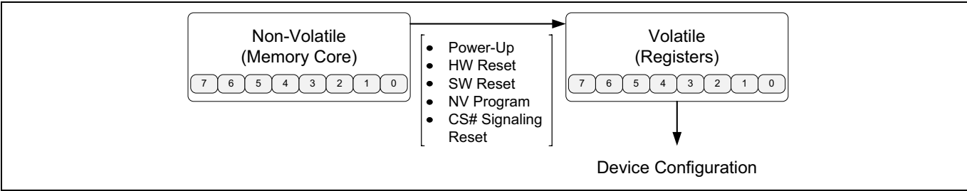
Figure 69 Data movement within register components
