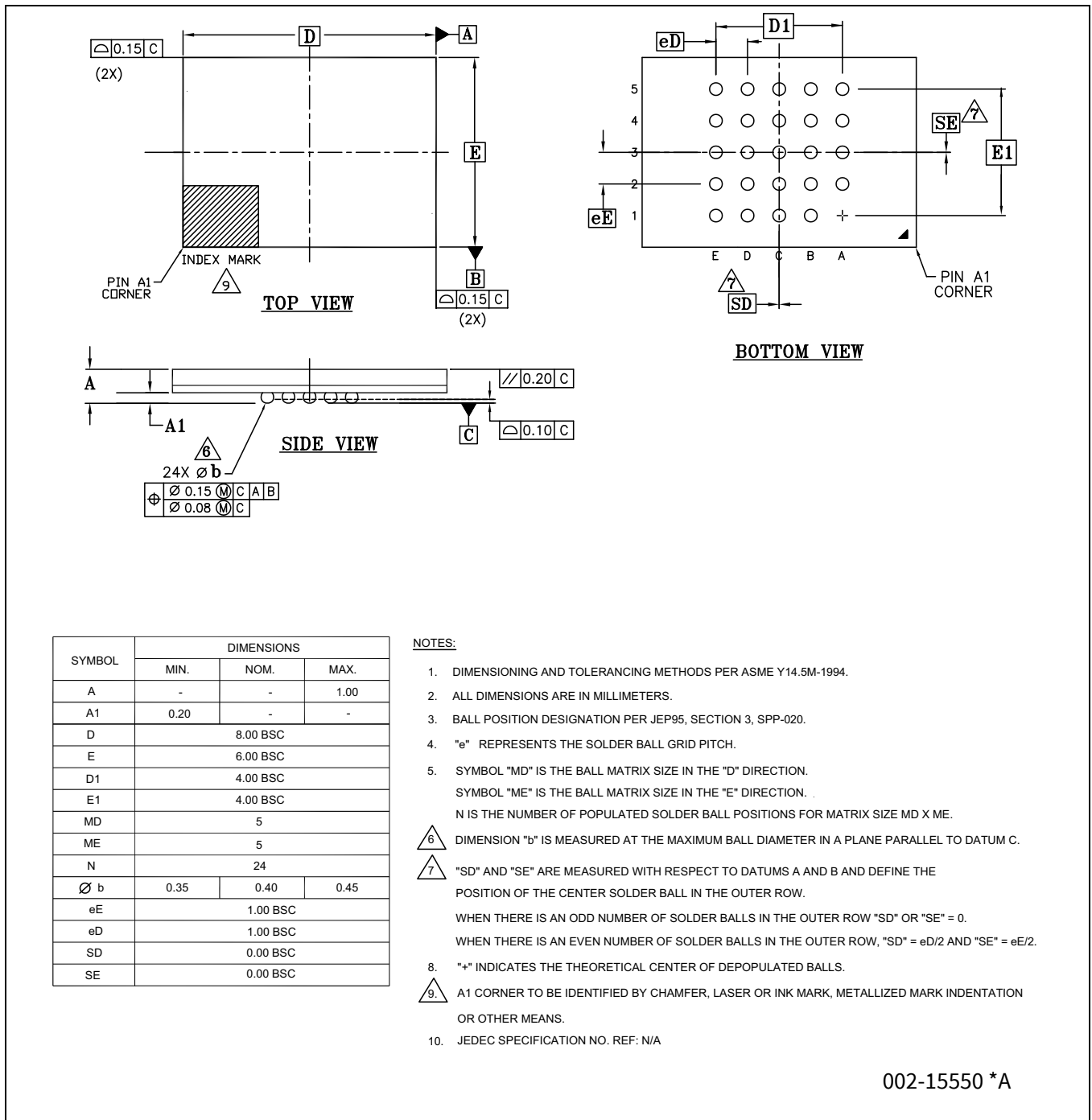
Figure 85 24-ball BGA (8.0 x 6.0 x 1.0 mm) package outline, 002-15550
