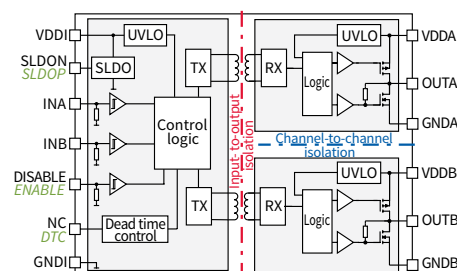
EiceDRIVER™ 2EDi product family device diagram
