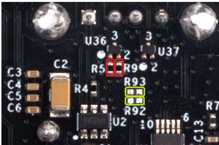
Figure 22 M.2 radio USB rework
