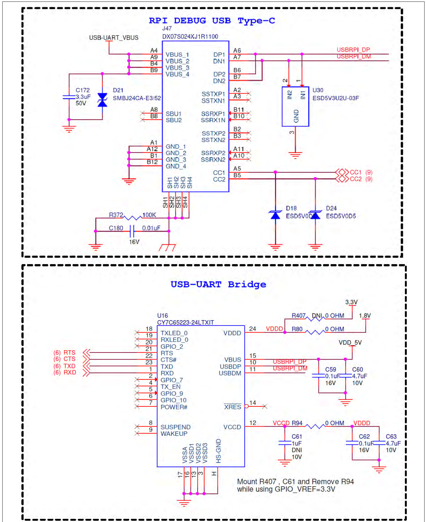
Figure 19 USB-UART bridge
