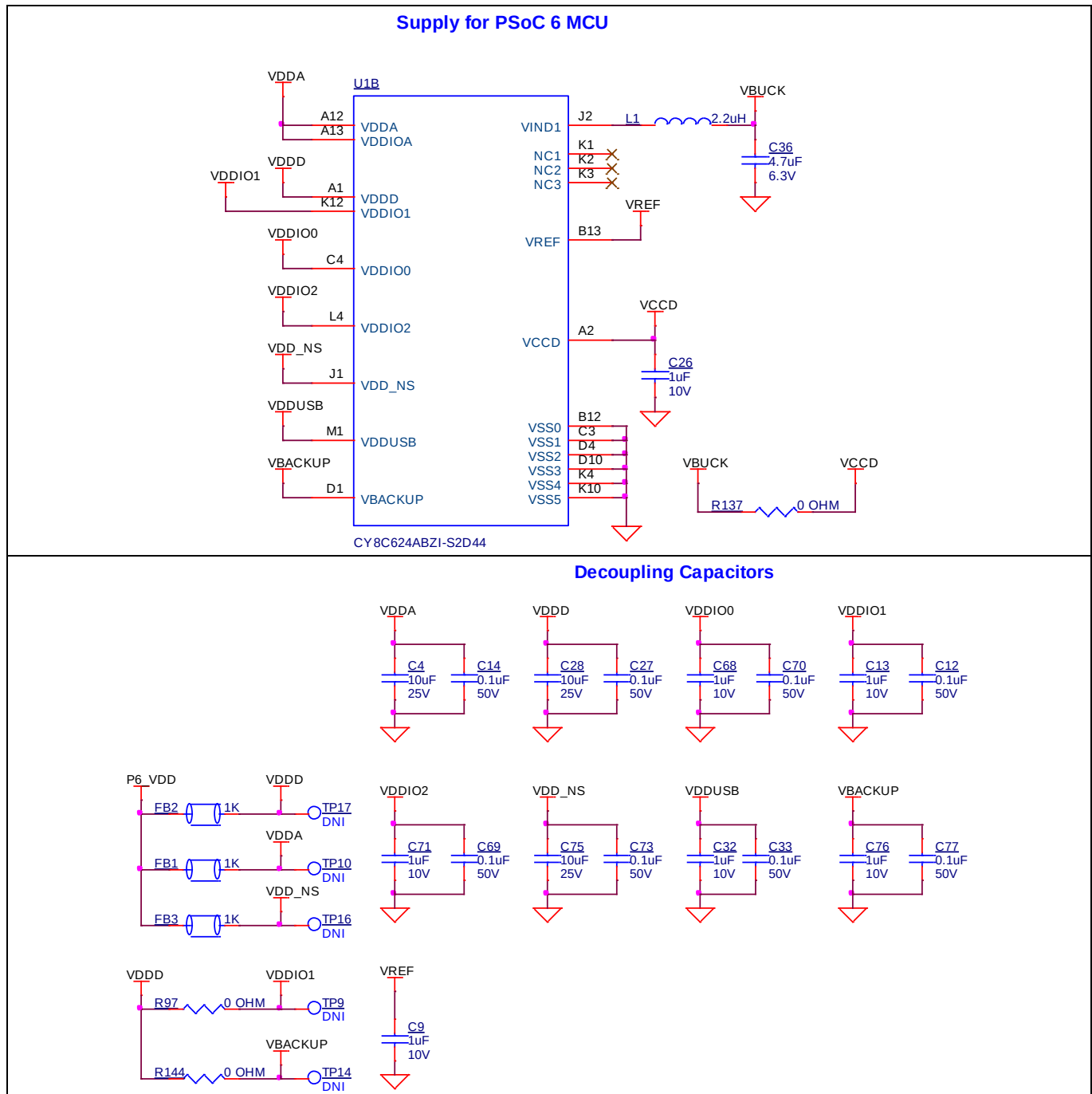
Figure 20 PSoC™ 6 MCU
