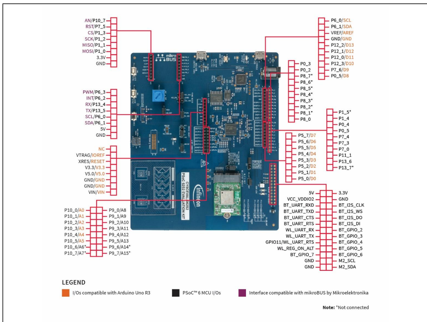
Figure 4 PSoC™ 62S2 evaluation board pinout
