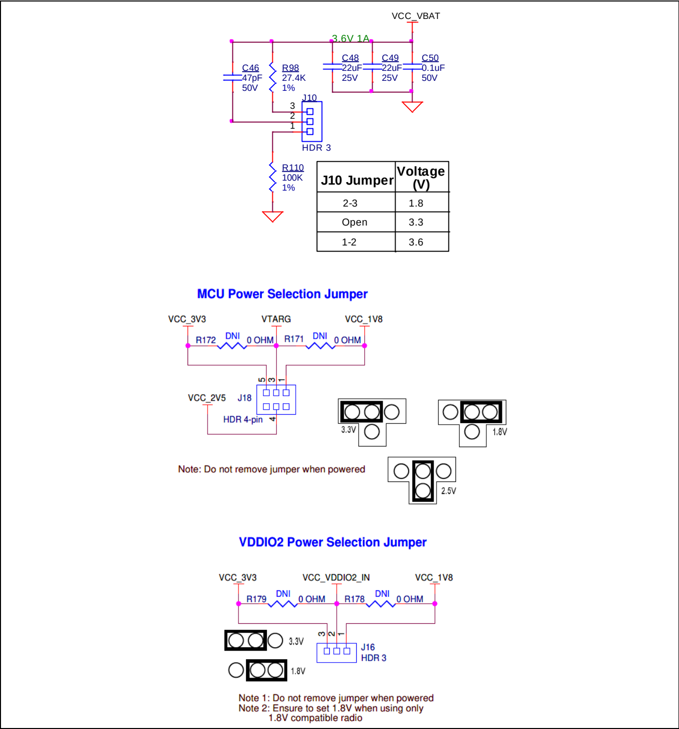
Figure 27 Voltage selection
