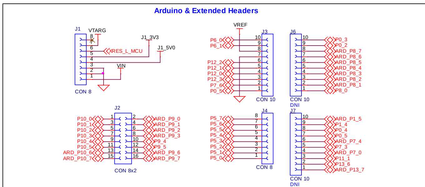
Figure 30 Headers compatible with Arduino Uno R3
