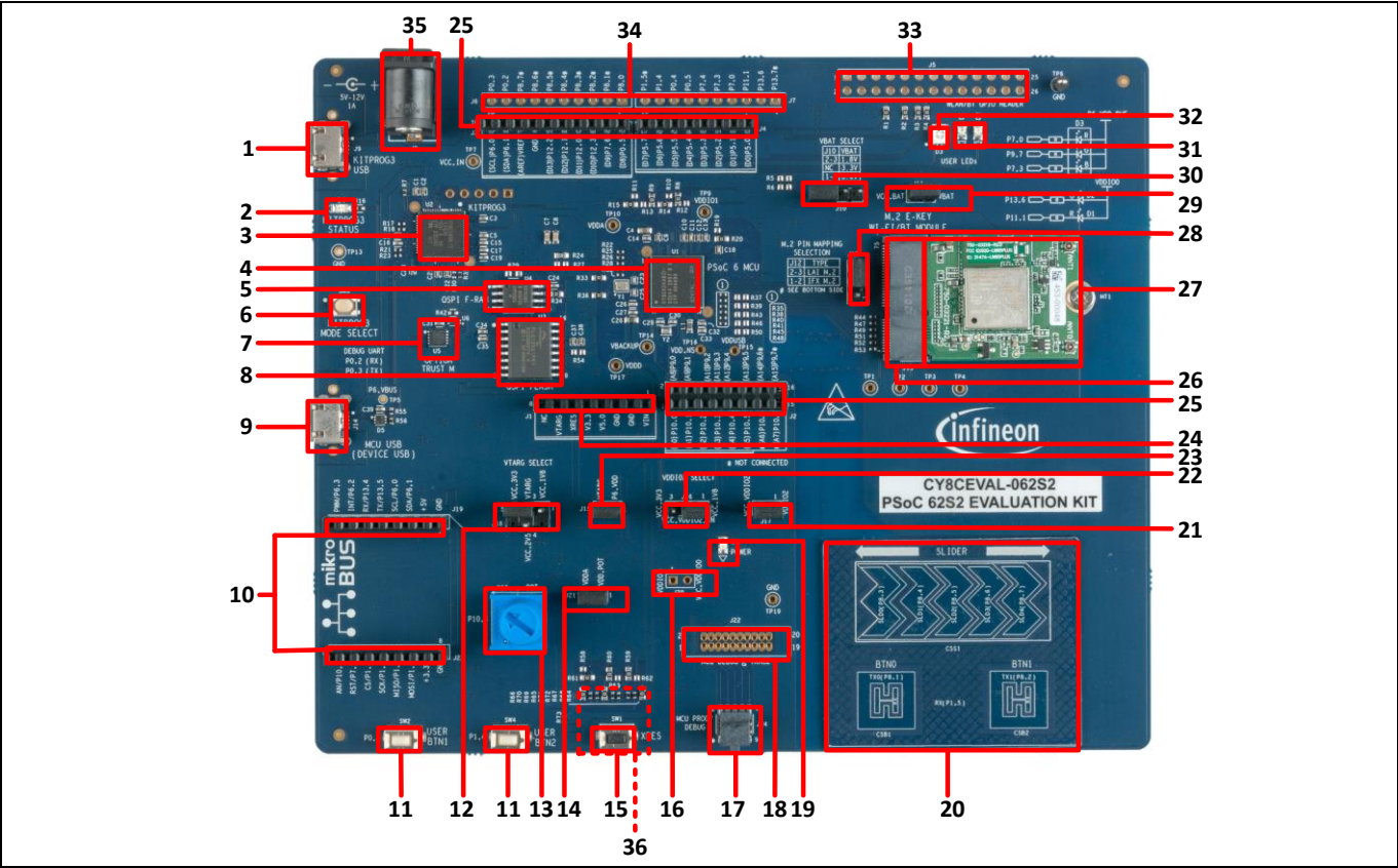
Figure 2 PSoC™ 62S2 evaluation board – top view
