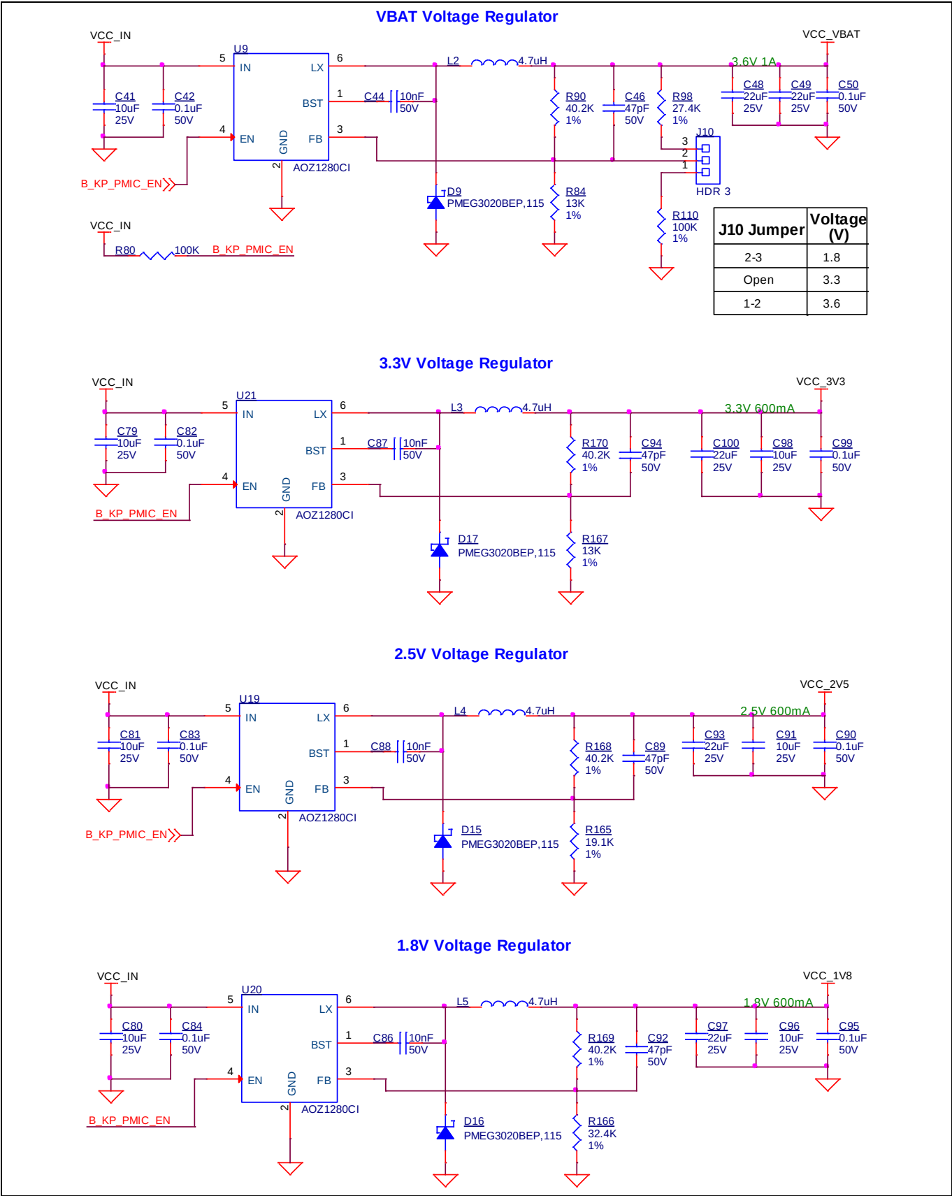
Figure 26 Voltage regulators
