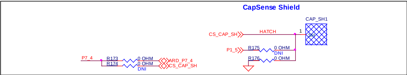
Figure 42 CAPSENSE™ shield
