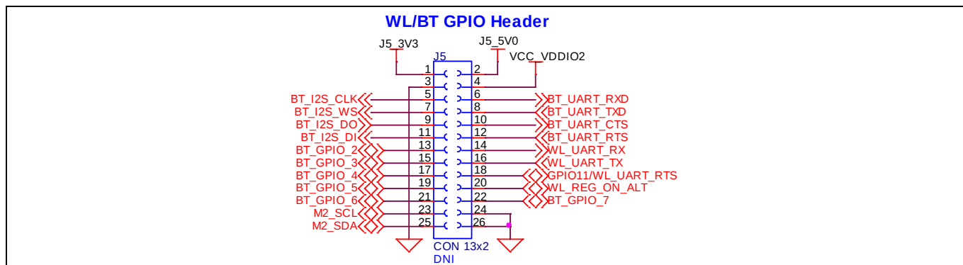
Figure 31 WLAN/BT GPIO header
