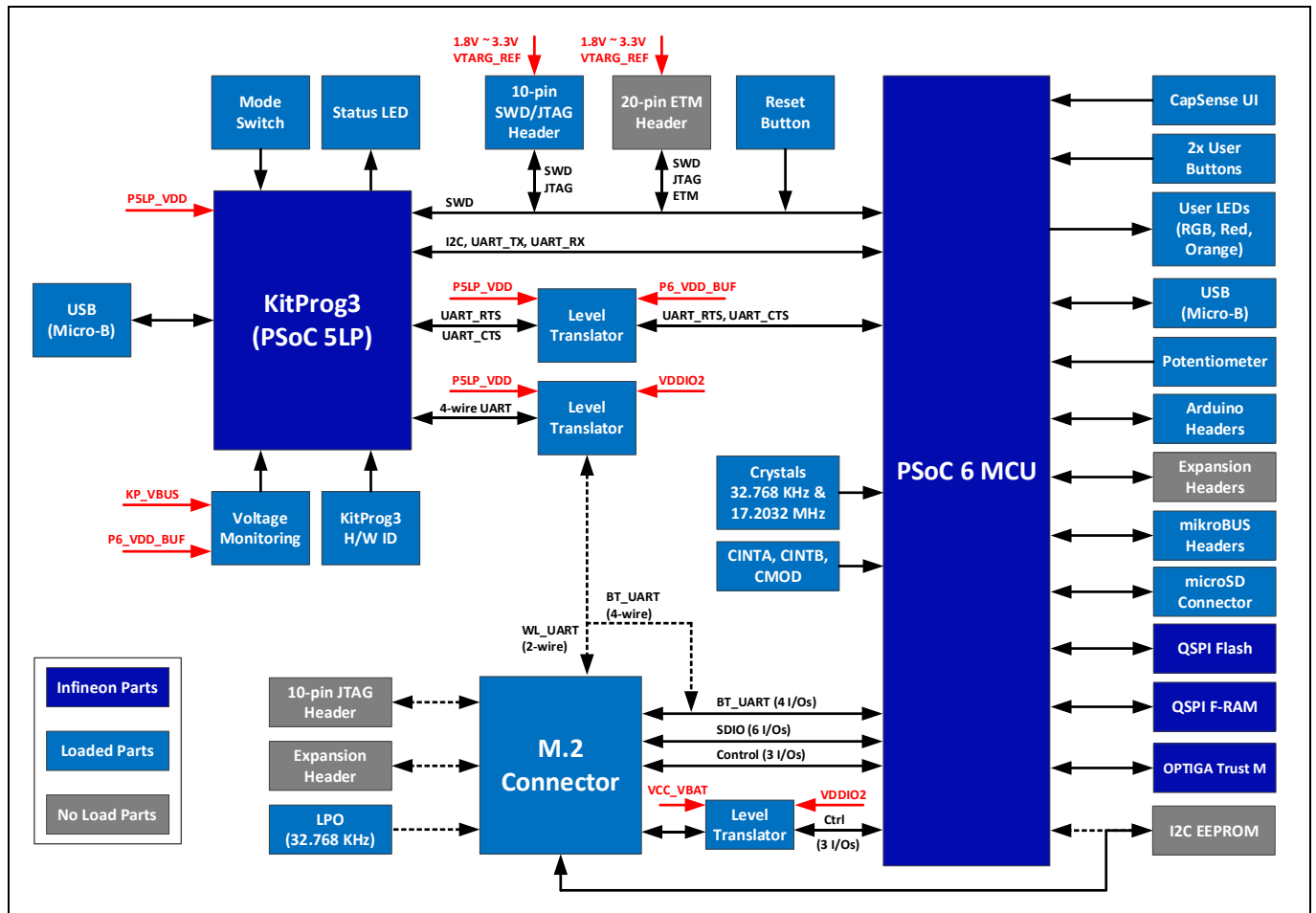
Figure 6 Block diagram of PSoC™ 62S2 evaluation board
