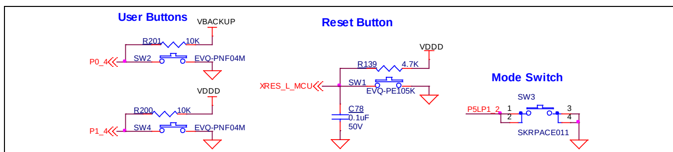
Figure 34 Push buttons
