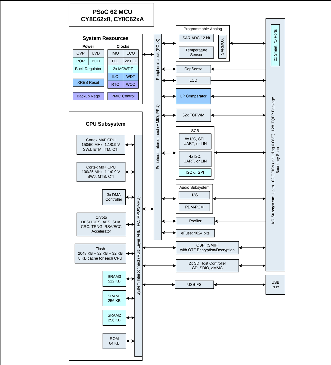
Figure 5 PSoC™ 62 MCU block diagram
