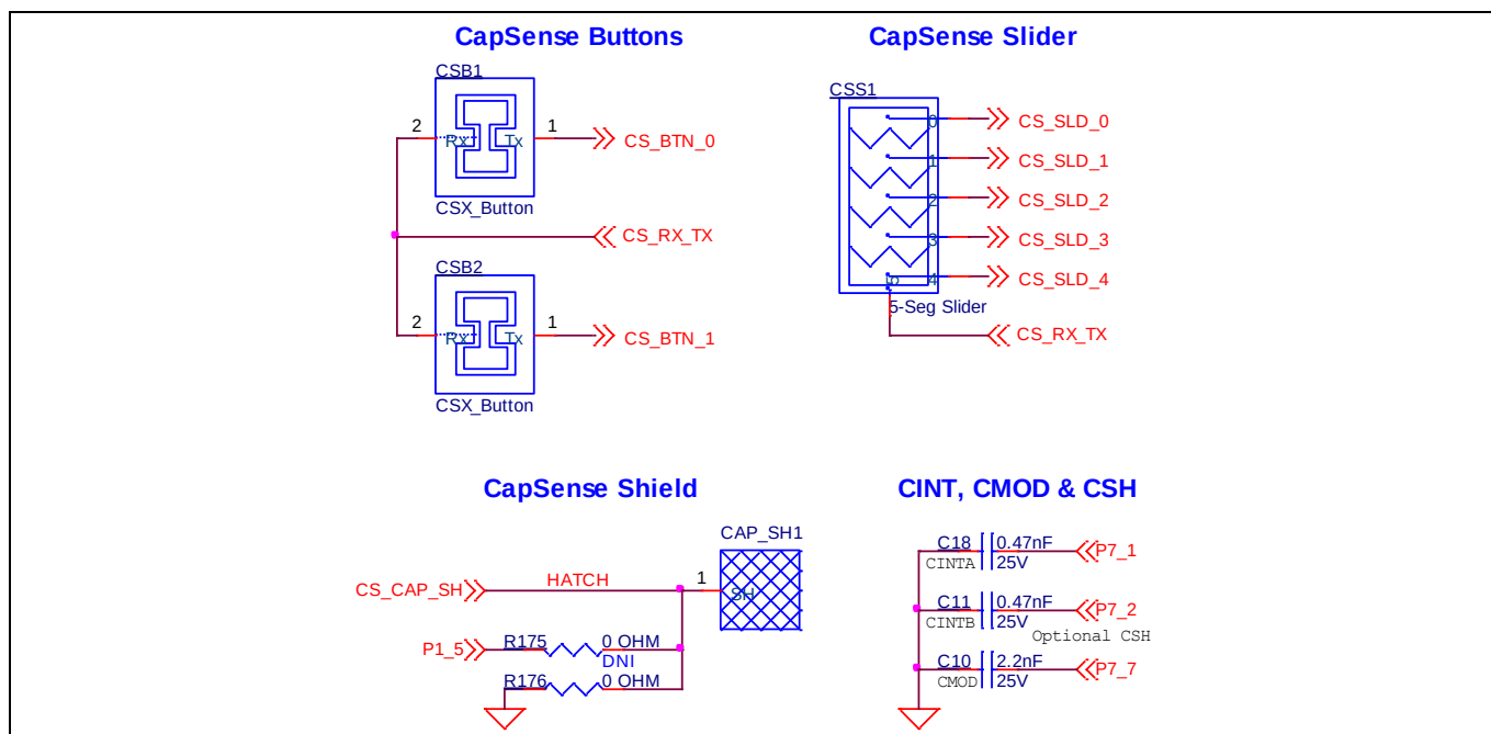
Figure 32 CAPSENSE™ circuit
