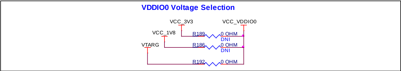
Figure 28 Voltage selection
