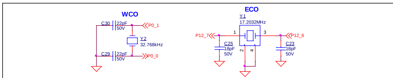
Figure 35 Crystal oscillators
