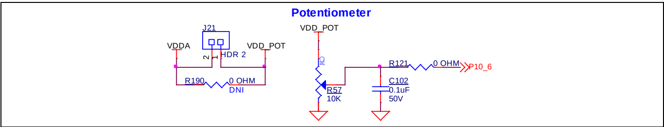
Figure 41 Potentiometer
