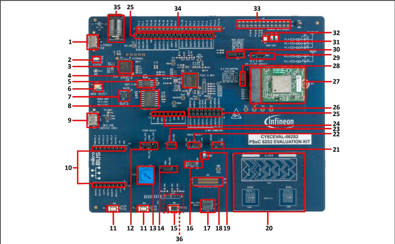
Figure 7 PSoC™ 62S2 evaluation board – top view
