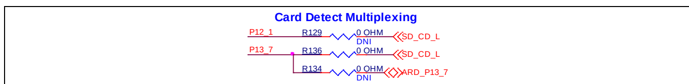
Figure 44 microSD card detect multiplexing
