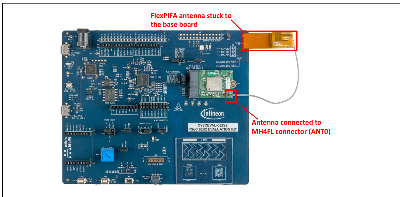
Figure 9 PSoC™ 62S2 evaluation board + Sterling-LWB5+ M.2 module from Laird Connectivity: Antenna connection
