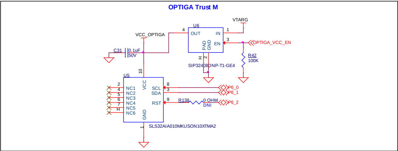
Figure 38 OPTIGA™ Trust M
