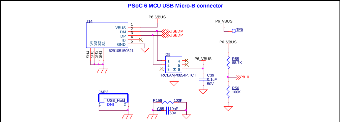
Figure 40 PSoC™ 6 MCU USB Micro-B connector
