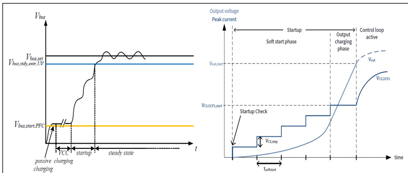
Figure 16 Start-up and shut-down parameters description
