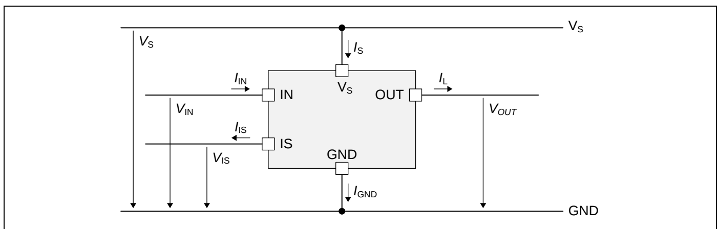
Figure 2 Definition of currents and voltages
