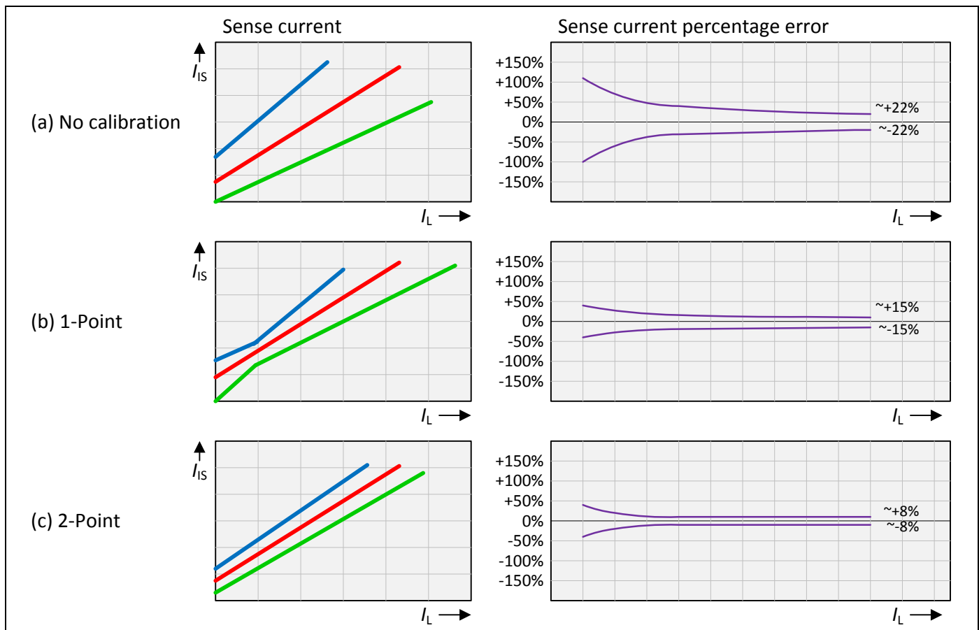
Figure 20 Accuracy of different calibration options
