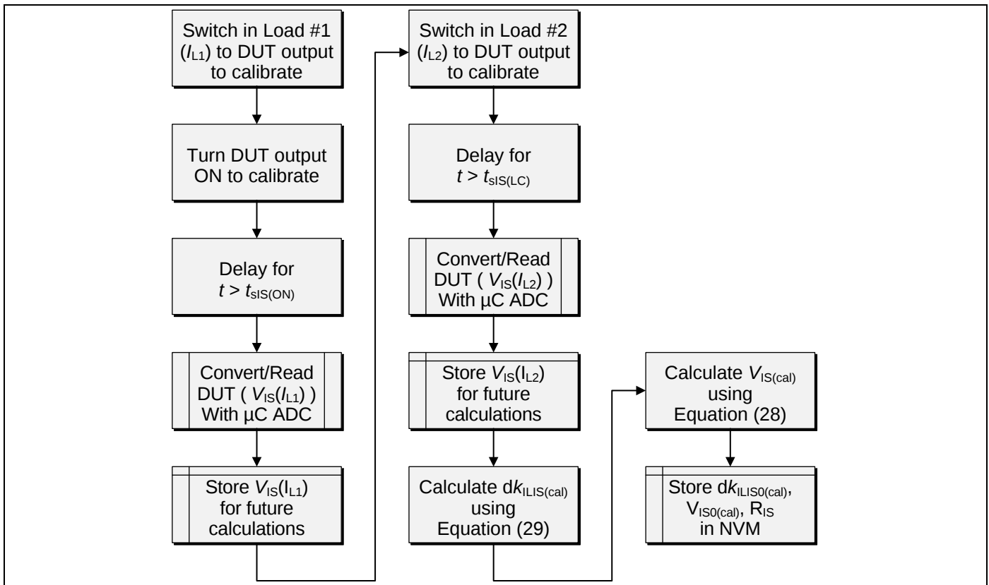
Figure 18 Manufacturing test procedure for the 2-Point calibration option
