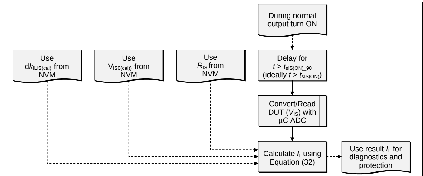
Figure 19 Application software procedure for the 2-Point calibration option
