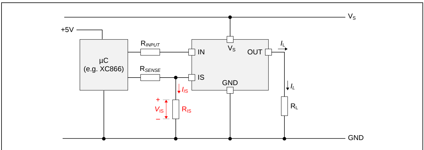
Figure 14 Reference circuit for calibration nomenclature
