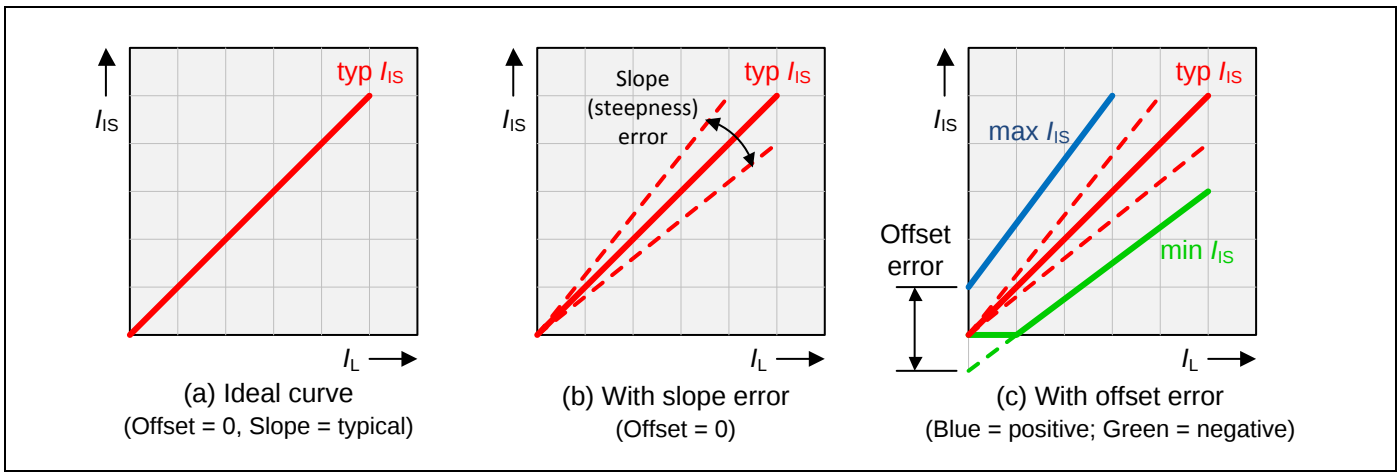
Figure 7 Relationship between I_{IS} and I_L in conventional devices
