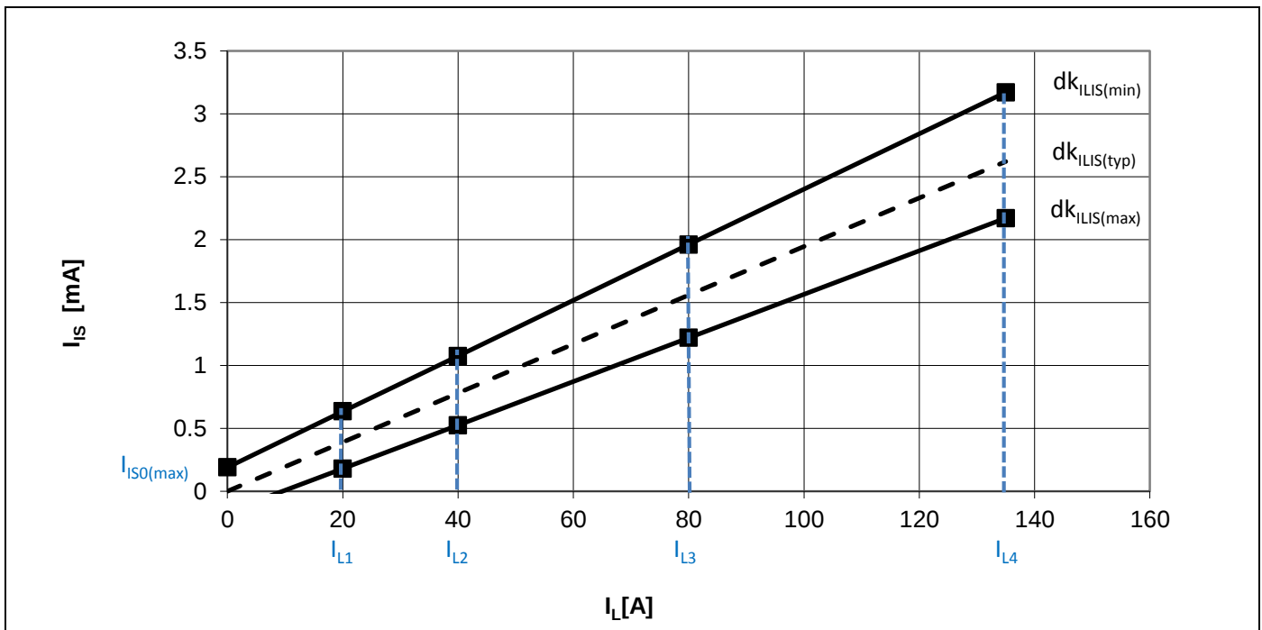
Figure 9 Power PROFET BTS50015-1TAD current sense
