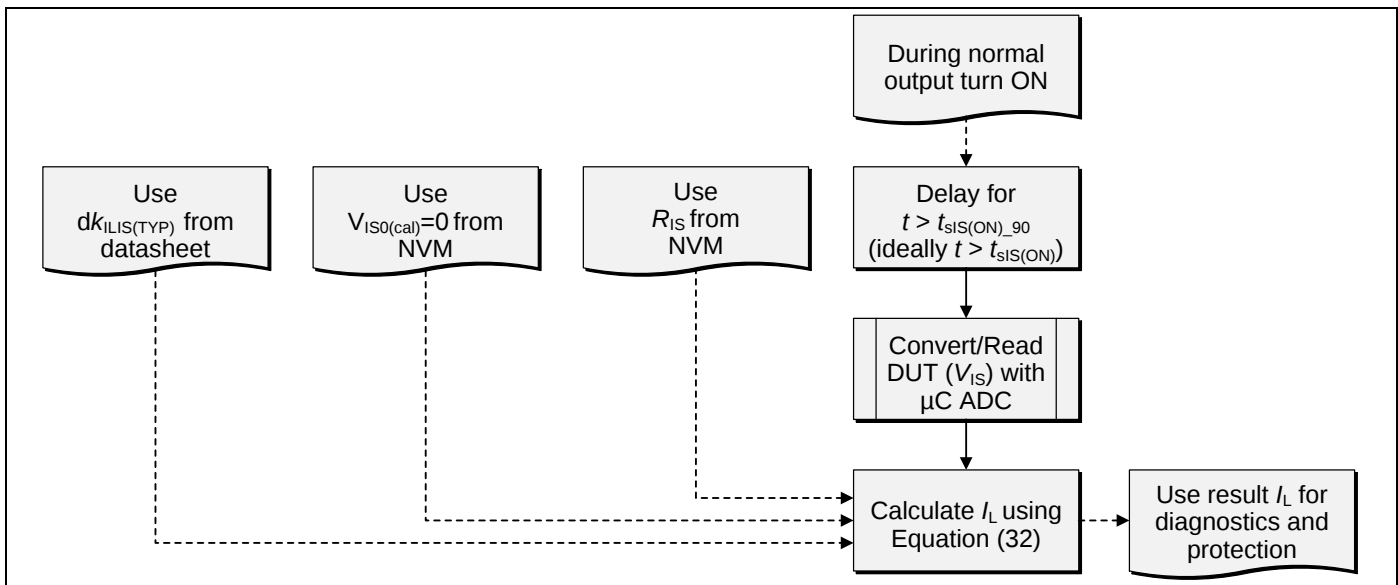
Figure 15 Application software procedure for No Calibration option
