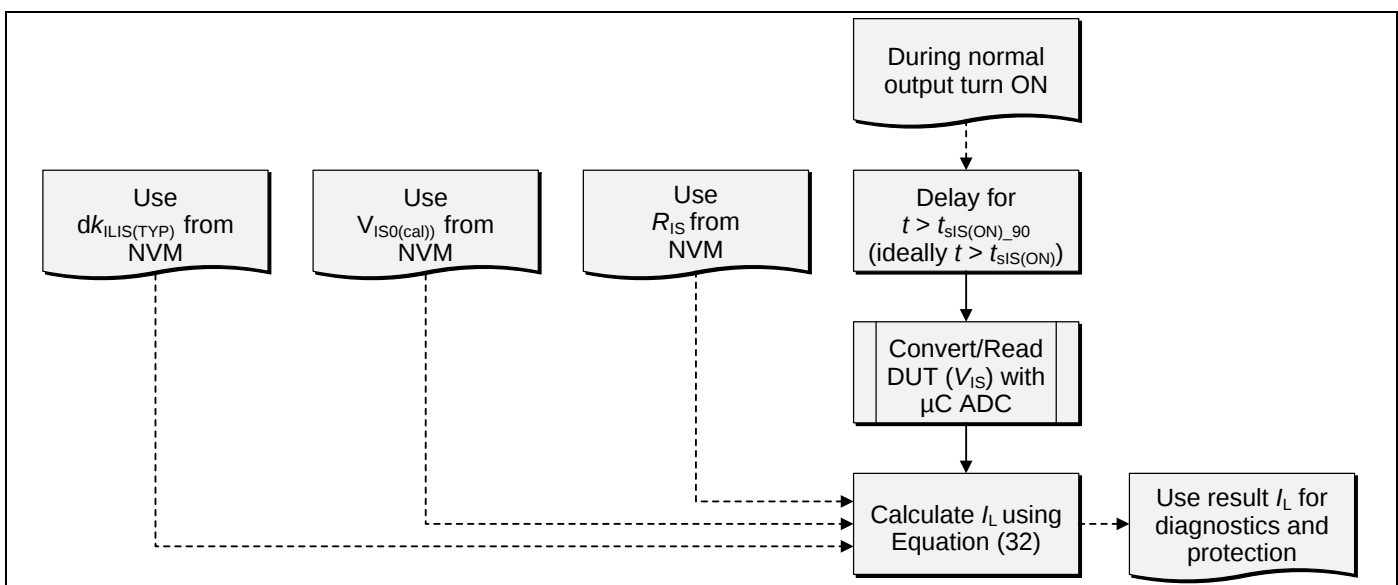
Figure 17 Application software procedure for the 1-point calibration option
