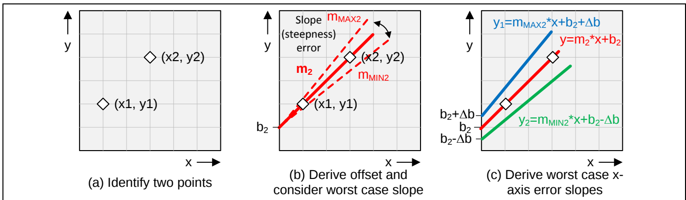
Figure 13 X-Axis error for generic lines with varying positive slopes and offsets
