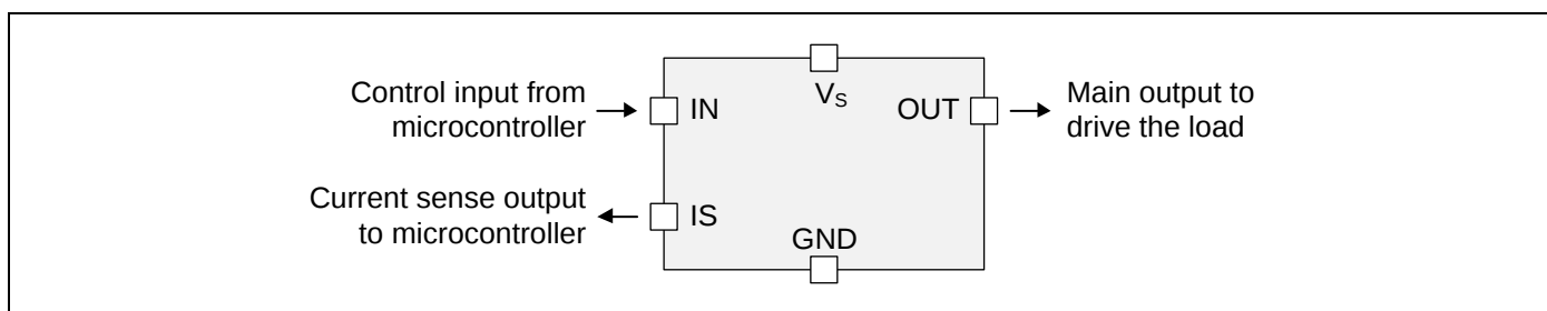
Figure 1 Pin names
