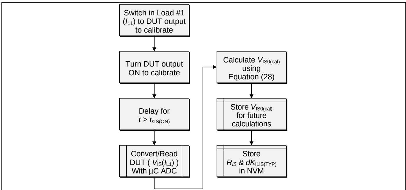
Figure 16 Manufacturing test procedure for the 1-point calibration option
