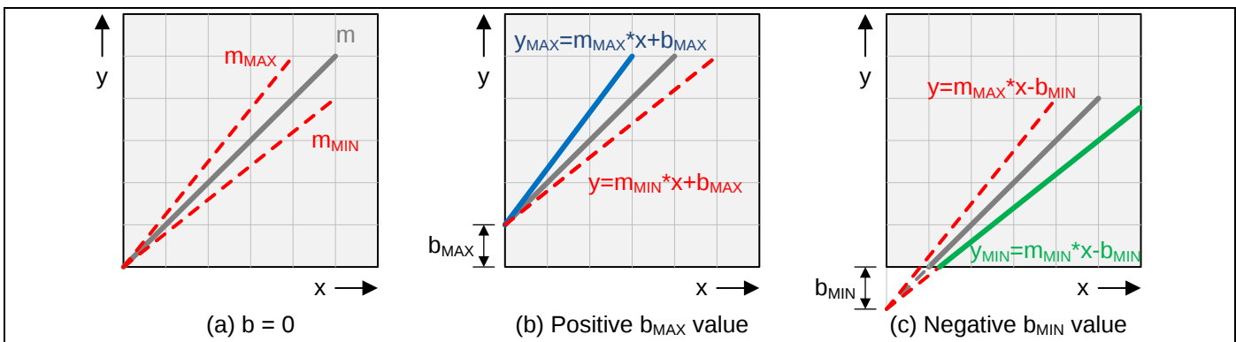
Figure 8 Generic lines with varying positive slopes
