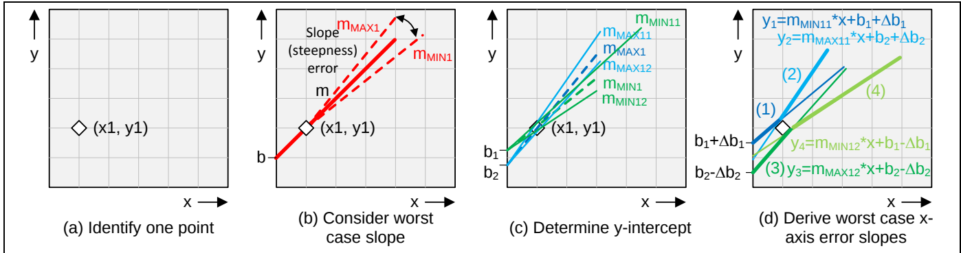
Figure 11 X-Axis error for generic lines with varying positive slopes and offsets
