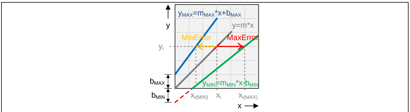
Figure 10 X-Axis error for generic lines with varying positive slopes
