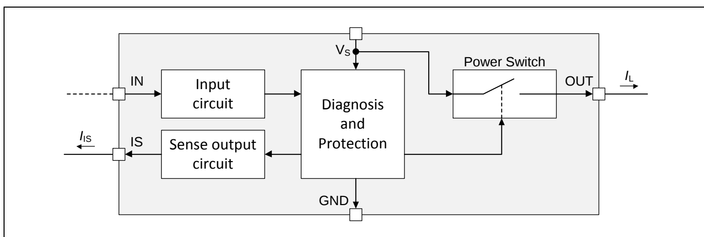
Figure 6 High-level block diagram for a conventional high-side power switch
