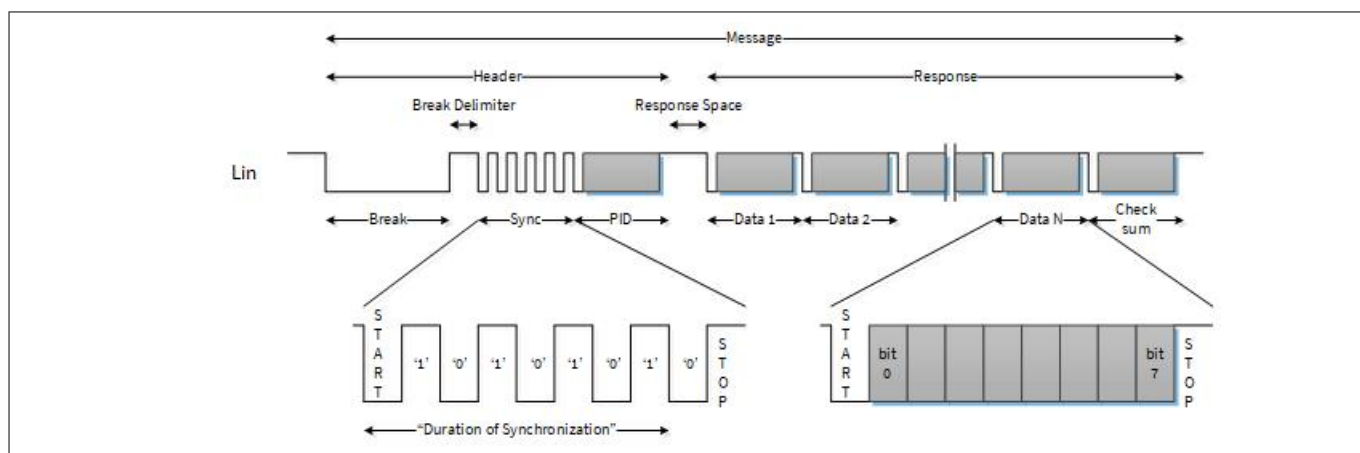
Figure 2 LIN Message Frame Format
