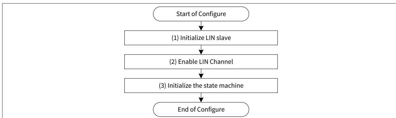
Figure 9 LIN Slave Initialize Flow Example
