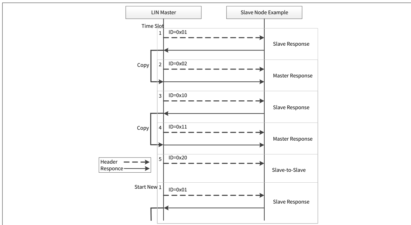
Figure 3 Communication Between LIN Master and Slave
