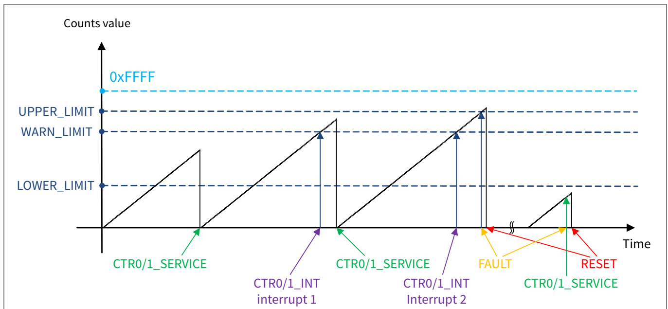
Figure 9 Subcounter 0/1 Operation in Window Mode with FAULT and RESET Action
