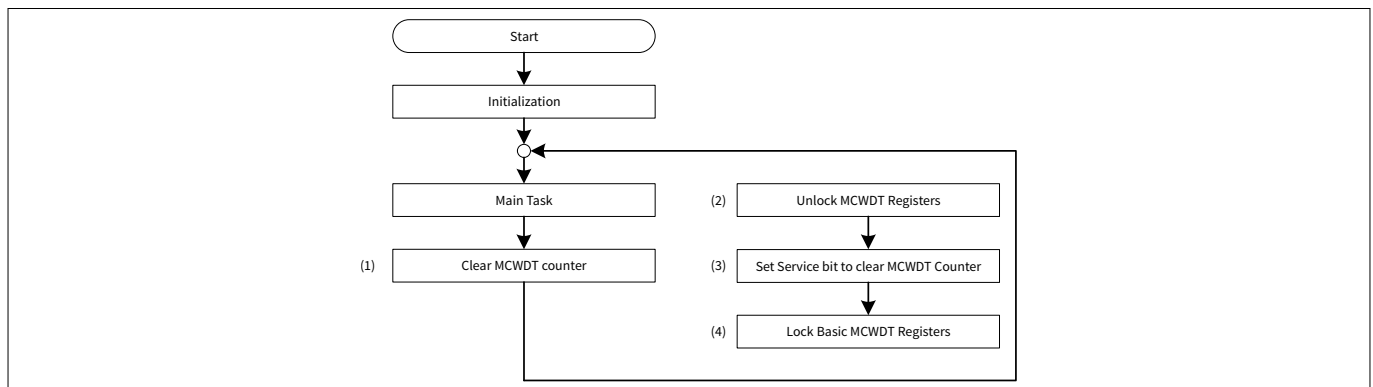
Figure 11 Example Flow to Clear MCWDT
