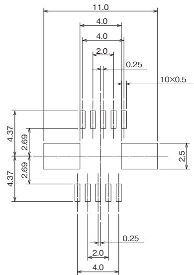
Recommended Metal Mask Pattern (t=0.15)
