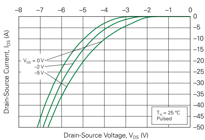
Fig. 11. Body Diode Curves @ T_{vj} = 25^\circ C
