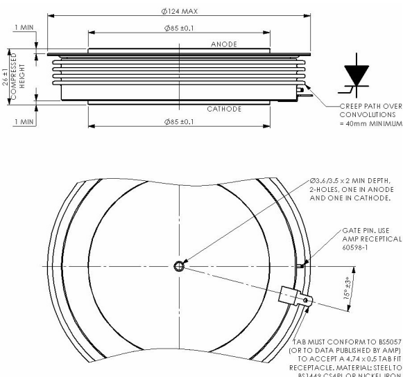
W107—101A411 EA Housing
