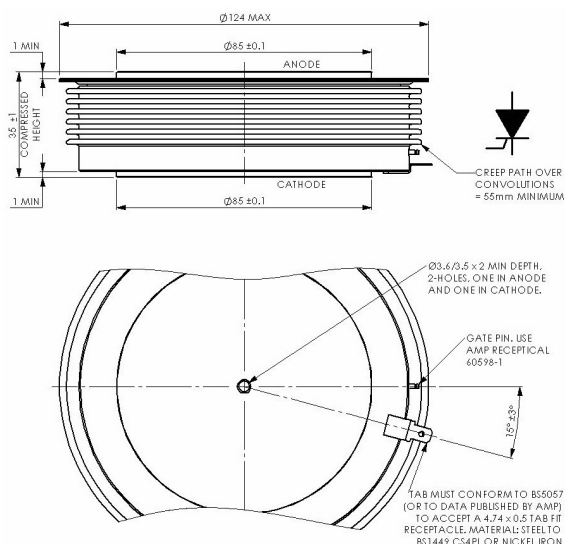
W108—101A410 EA Housing
