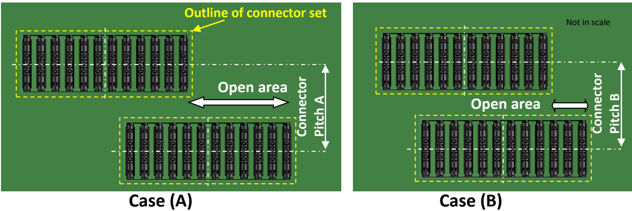
Figure 5-28 Parallel nounting
