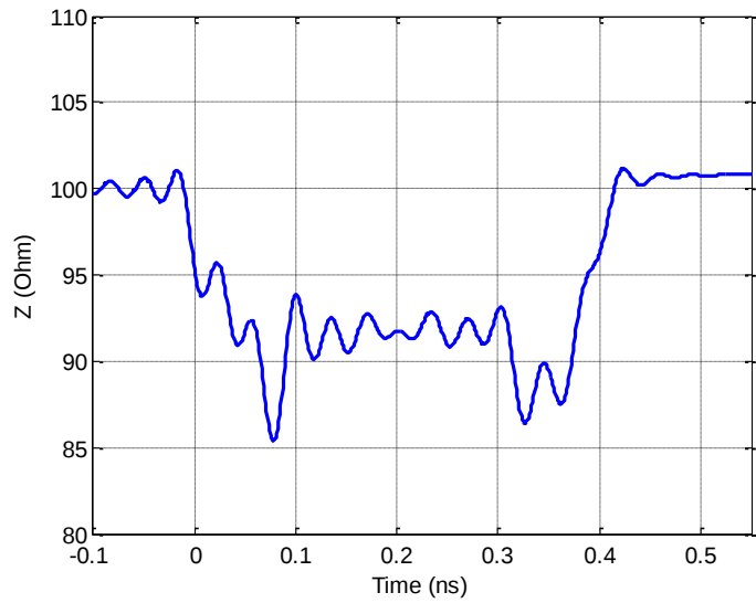
Figure 4-15 Simulated differential impedance of IT8-35mm @12ps (20-80%) rise time
