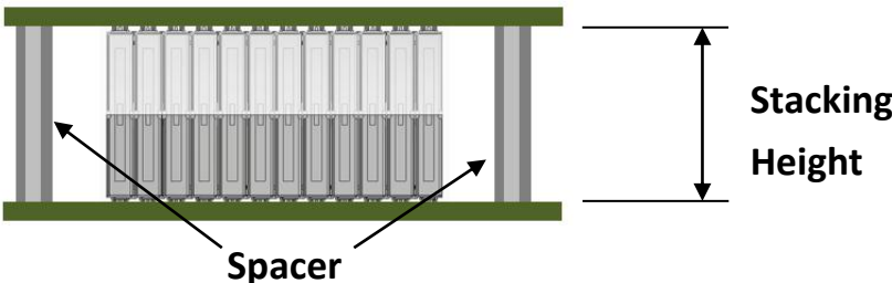
Figure 5-25 Spacers
