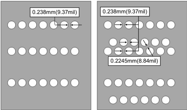
Routing example 1
