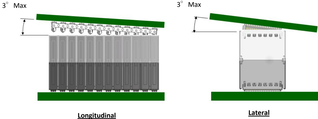
Figure 6-9 Angles During Manual Disassembly
