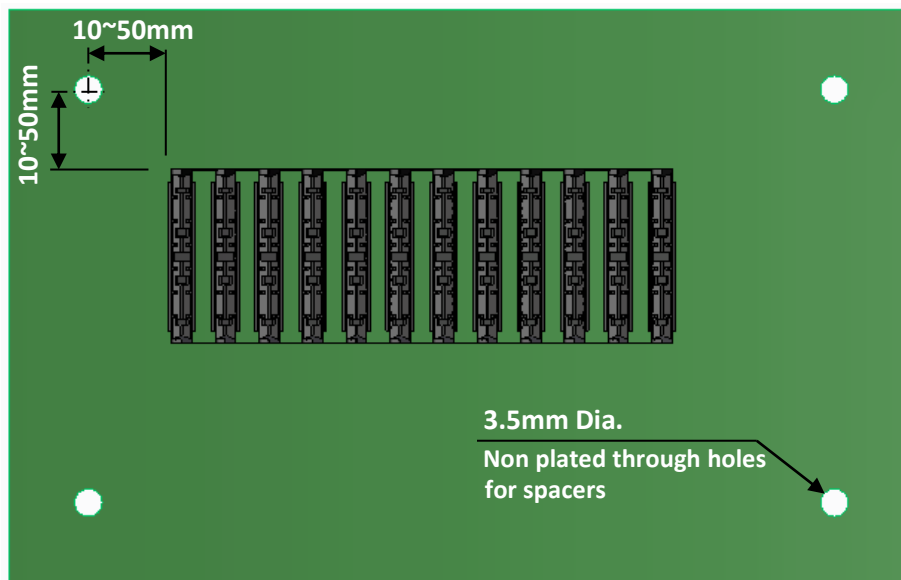
Figure 5-27 Spacer location
