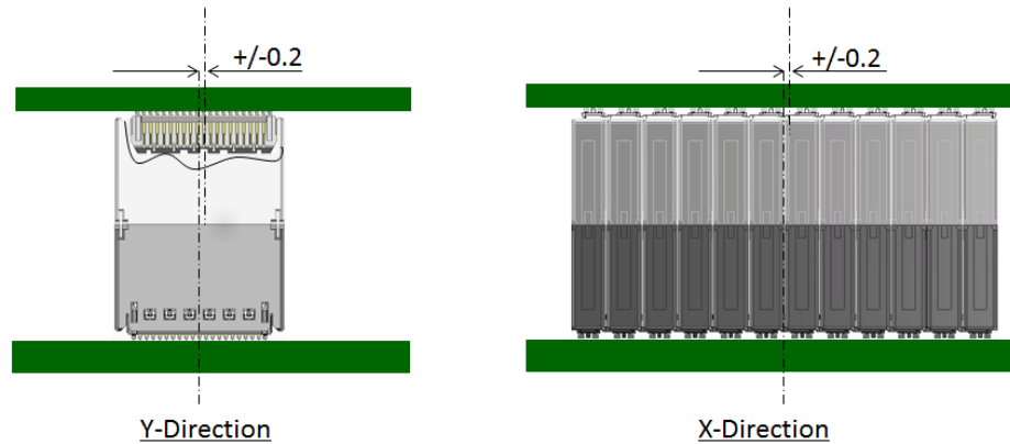
Figure 5-36 Mating tolerances
