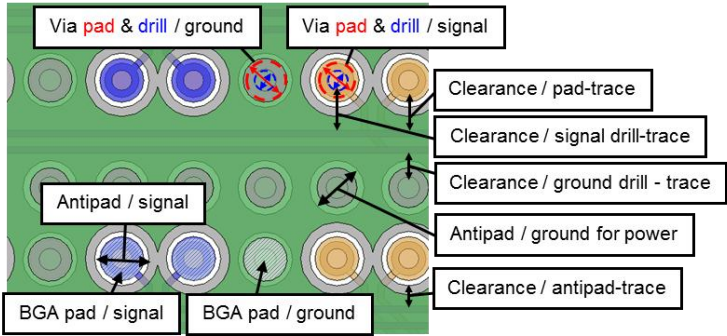
Figure 5-20 Routing Example 6: Via-in-Pad with additional ground vias between all columns
