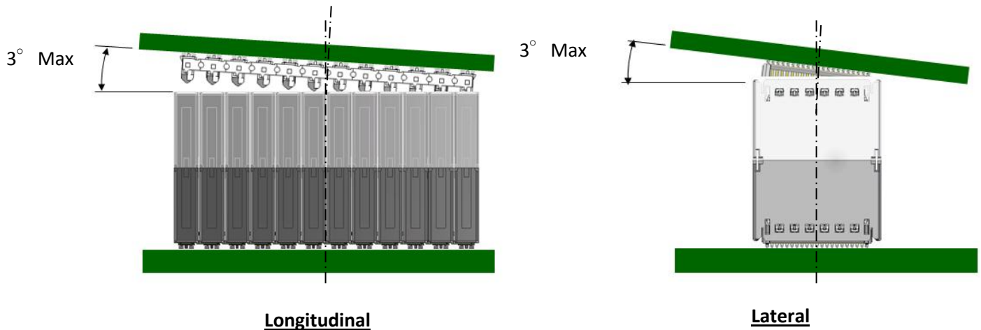
Figure 6-5 Angles During Manual Installation
