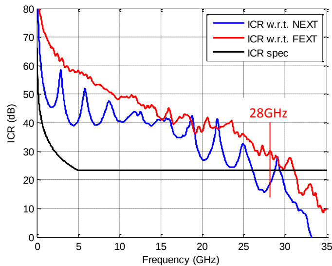
Figure 4-5 IT8-35mm insertion loss to crosstalk ratio
