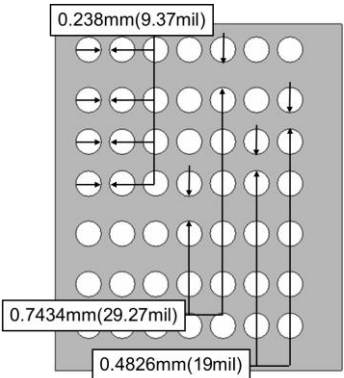
Figure 5-21 Power plane view of routing example 6
