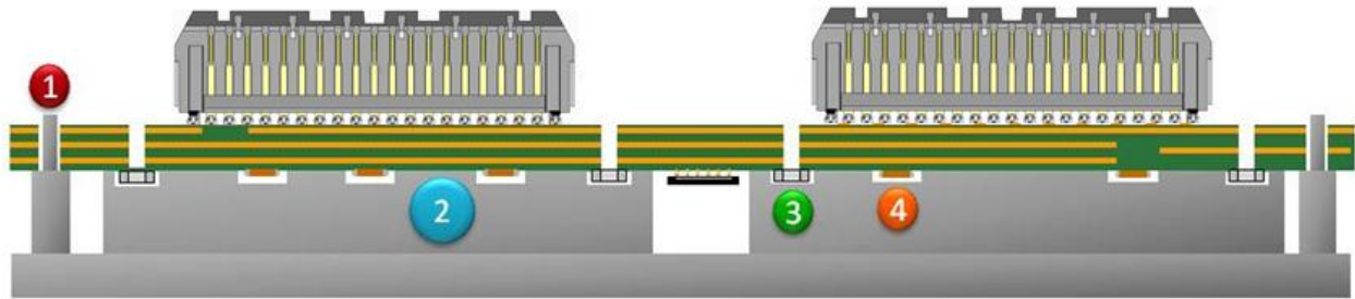
Figure 6-4 System Assembly Support Fixture
