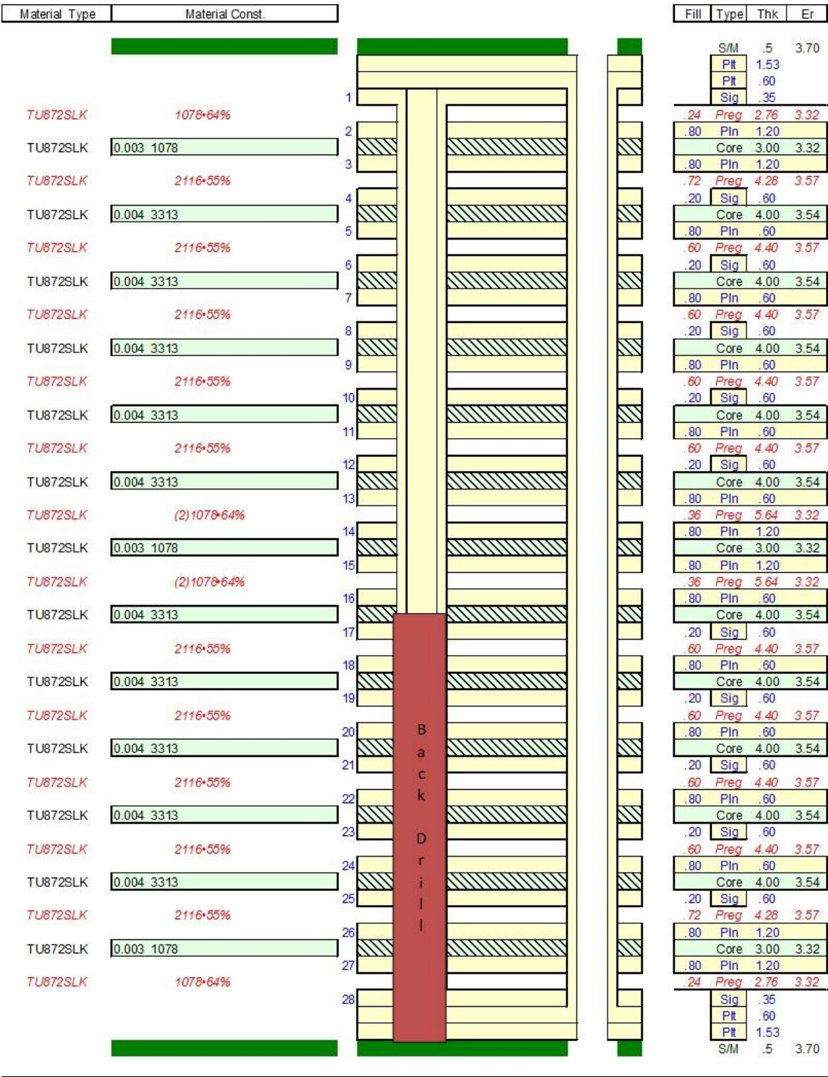
Figure 5-22 PCB stack up example
