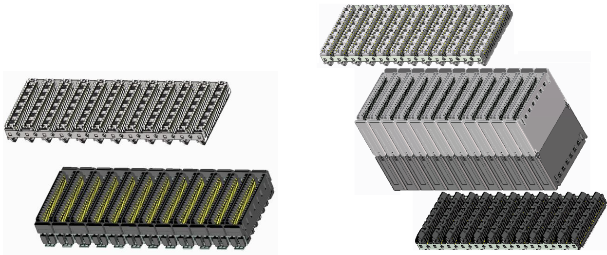
Stack Height 14mm ~46mm Three-piece type
