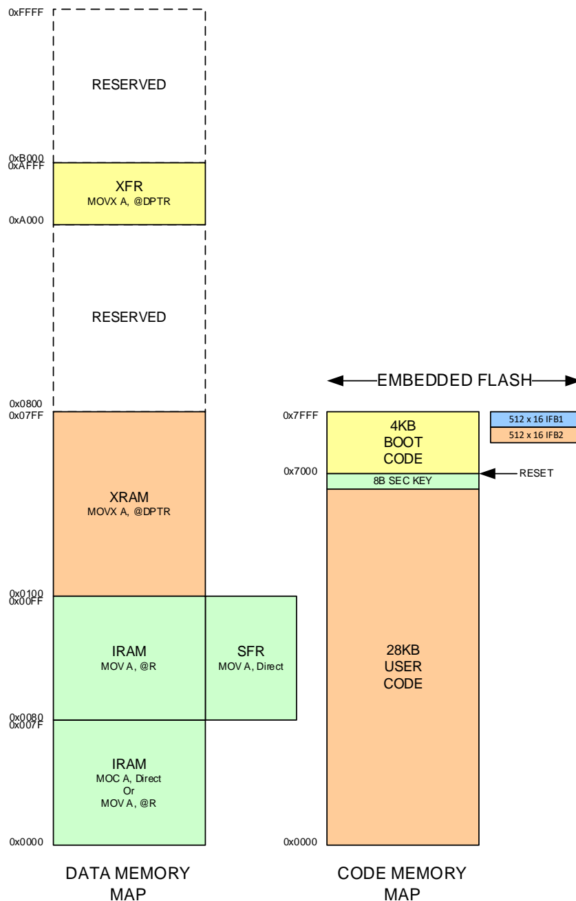
Figure 2-1 Memory Map
