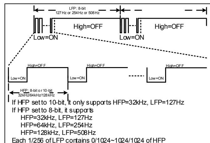
Figure 8 PWM Timing Diagram
