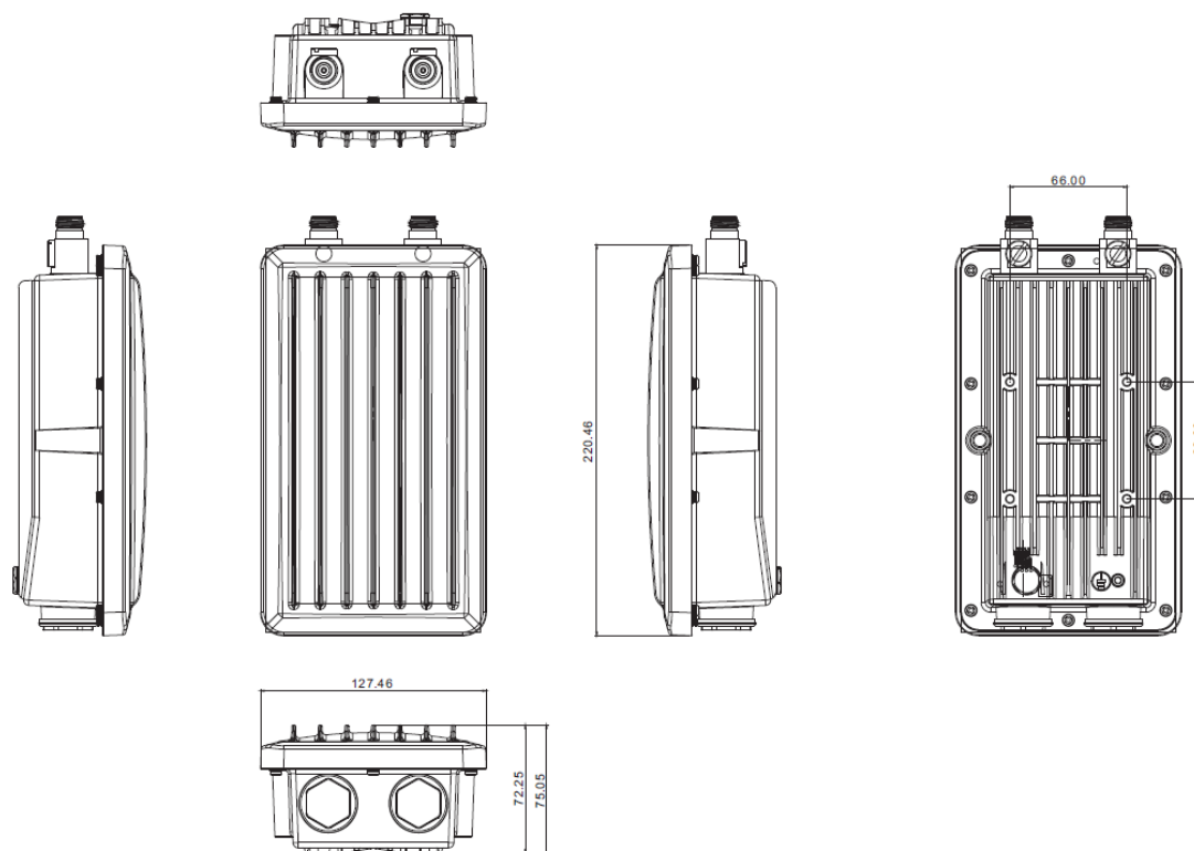
IGAP-W612H+ Wall-mounting Measurements (Unit = mm)
