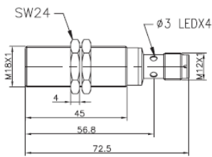
Fig. 16 Flush version, plug
