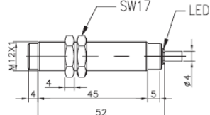
Fig. 11 Non-flush version, cable
