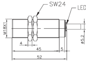
Fig. 14 Flush version, cable
