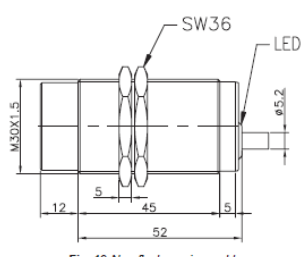
Fig. 19 Non-flush version, cable
