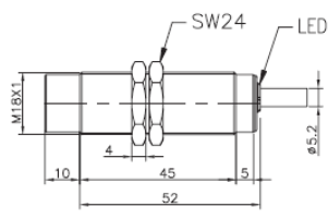
Fig. 15 Non-flush version, cable
