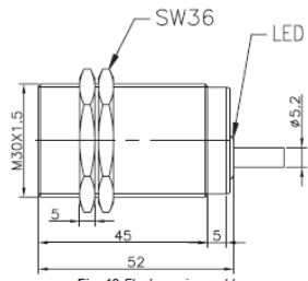
Fig. 18 Flush version, cable
