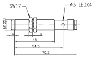
Fig. 13 Non-flush version, plug
