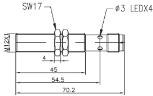
Fig. 12 Flush version, plug
