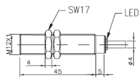
Fig. 10 Flush version, cable
