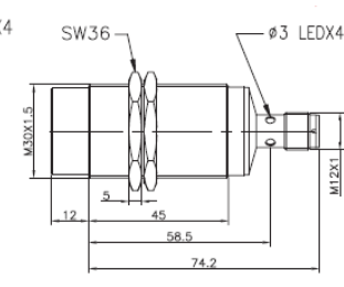
Fig. 21 Non-flush version, plug
