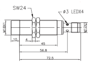
Fig. 17 Non-flush version, plug
