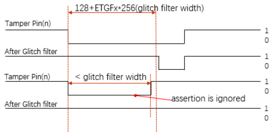
Figure 1. Glitch filter working
