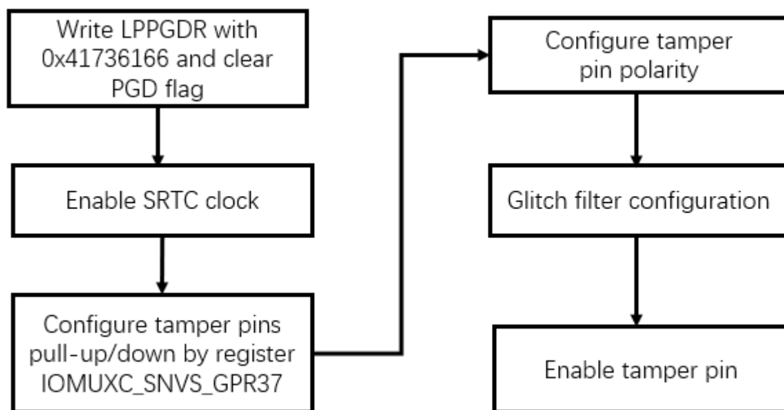
Figure 2. Passive tamper initialization flow
