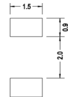
Figure 6: Recommended Soldering Land Pattern
