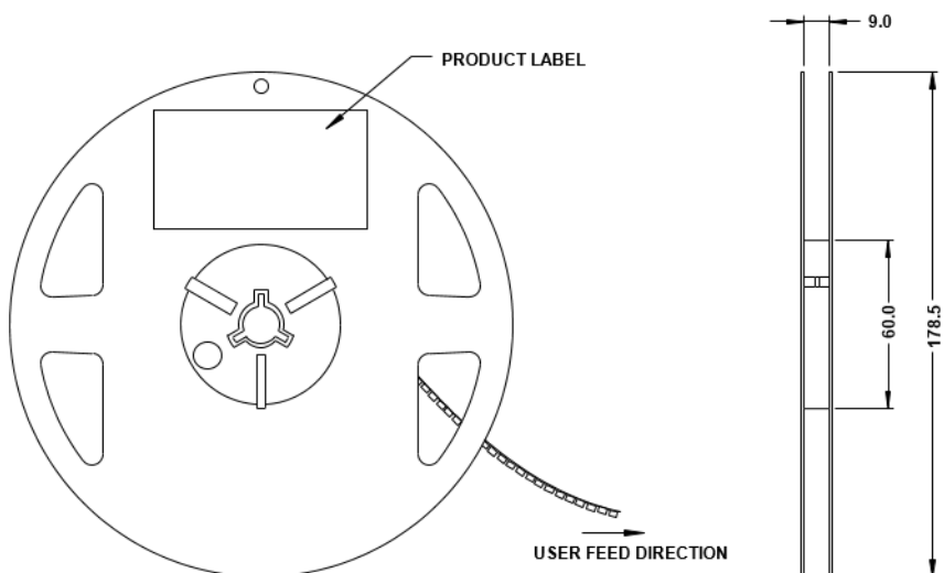
Figure 8: Reel Dimensions
