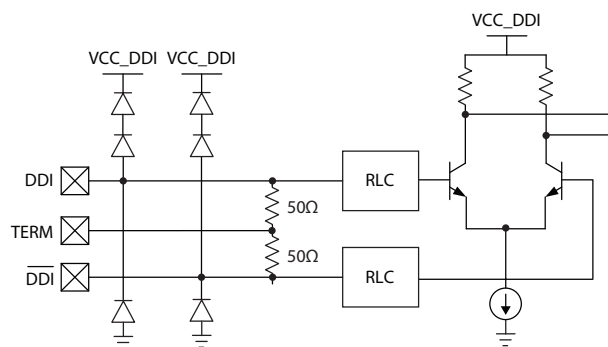
Figure 3-1: DDI/ \overline{\text{DDI}}
