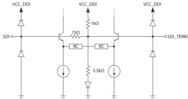
Figure 3-2: SDI/SDI_TERM
