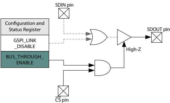
Figure 4-23: GSPI_BUS_THROUGH_ENABLE Operation
