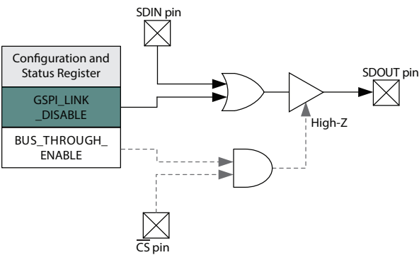
Figure 4-22: GSPI_LINK_DISABLE Operation
