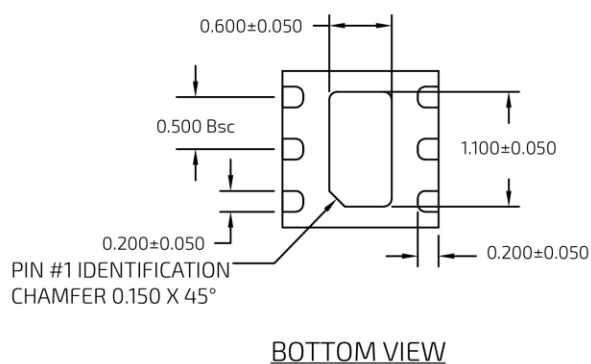
1.5 x 1.5 mm DFN-6 Package Dimensions
