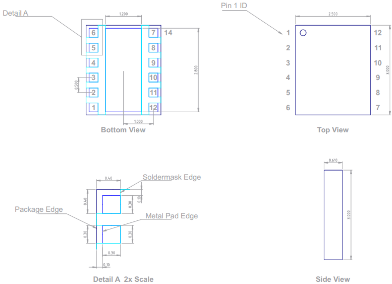
LAMM12 2.5x3.0mm Dimensions in millimeters
