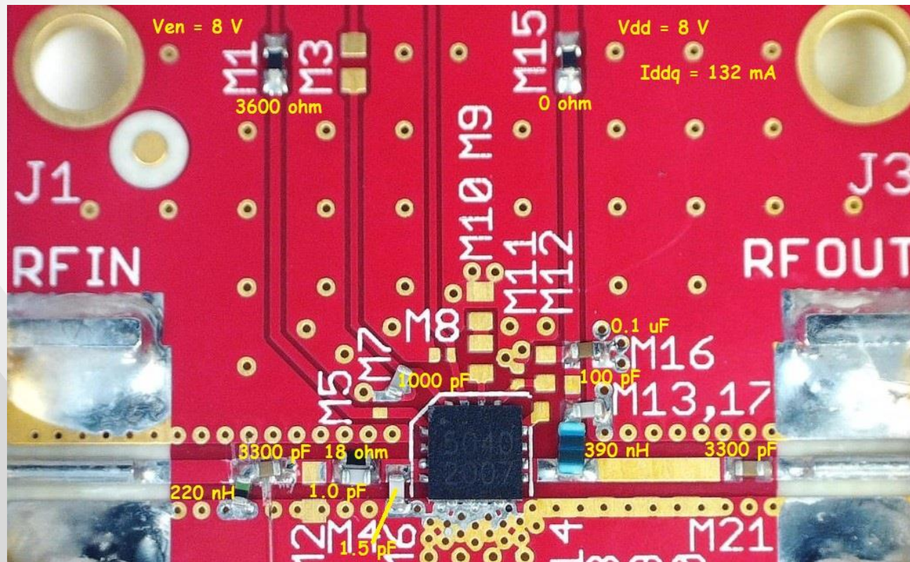
GRF5040 Eval Board # 200 (100-800 MHz)
