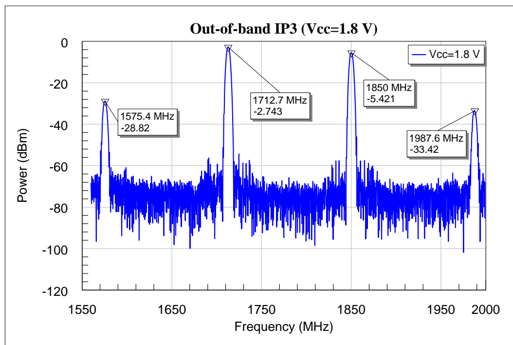
Figure 19 Out-of-band IP3 of the BGA524N6 as LNA for GNSS applications (1.8V)
