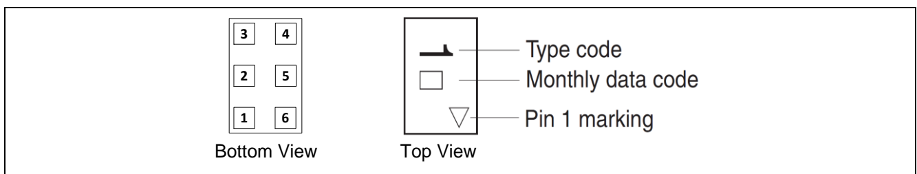
Figure 3 Package and pin connections of BGA524N6
