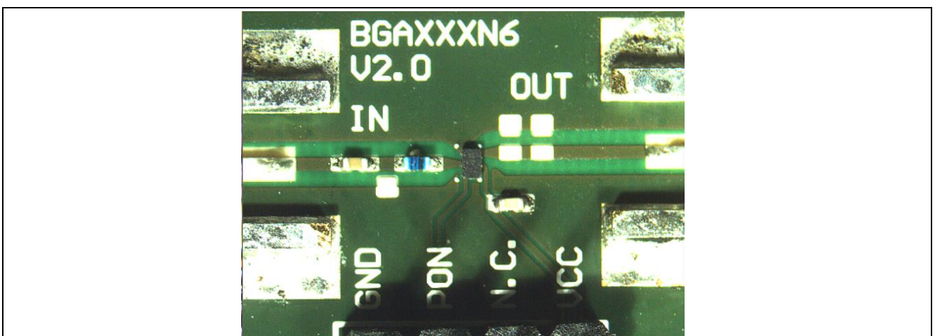
Figure 24 Photo Picture of Evaluation Board (detailed view)
