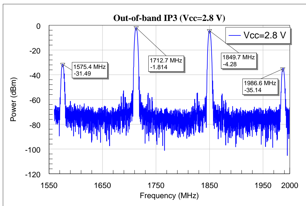
Figure 20 Out-of-band IP3 of the BGA524N6 as LNA for GNSS applications (2.8V)
