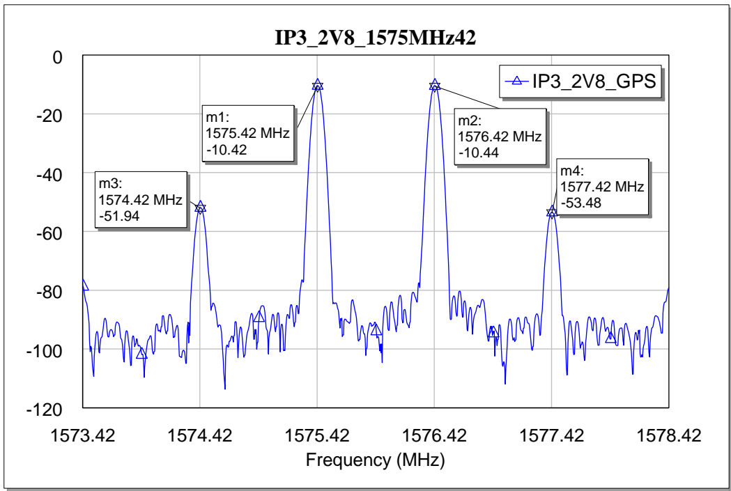
Figure 18 Output IP3 of the BGA524N6 as LNA for GNSS applications (2.8V)
