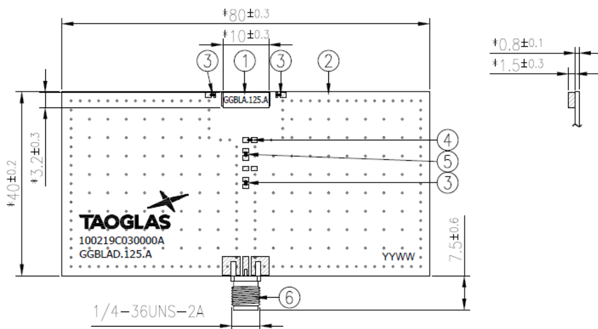
Back View
