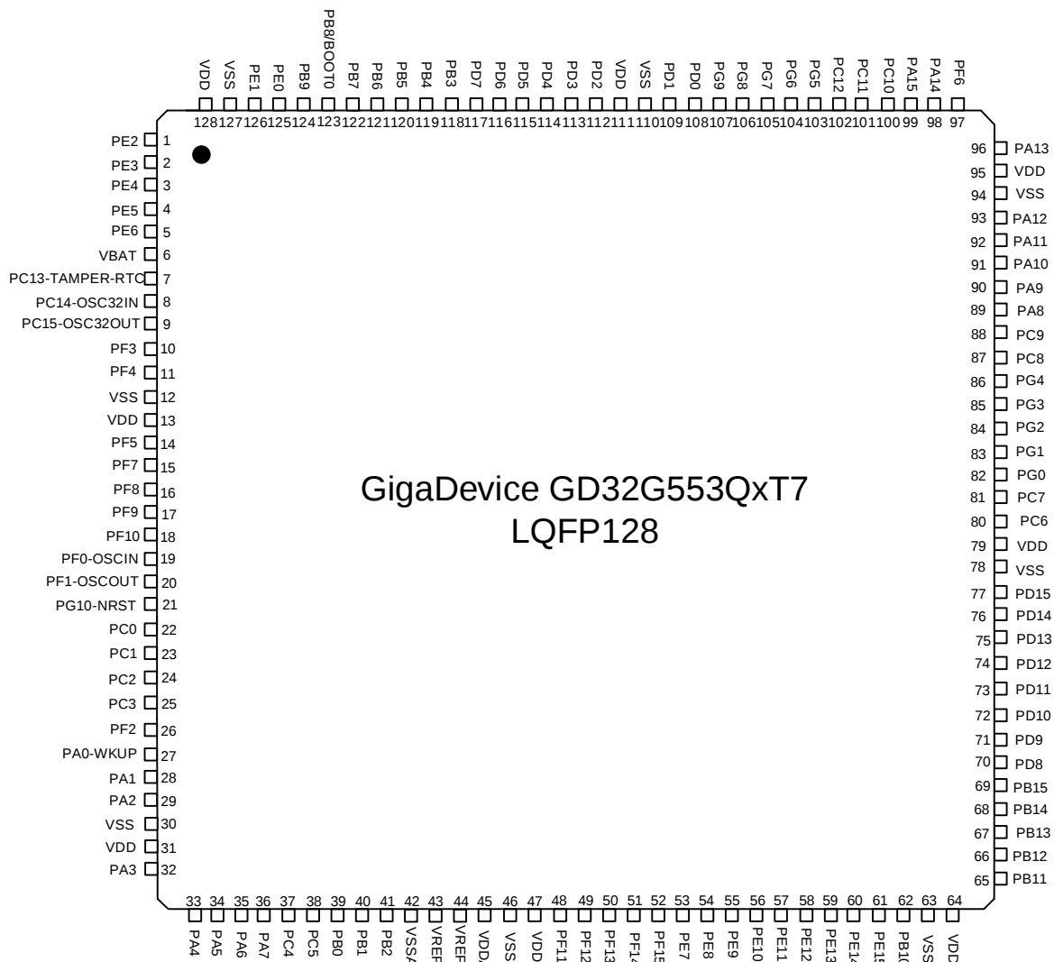
Figure 2-2. GD32G553QxT7 LQFP128 pinouts
