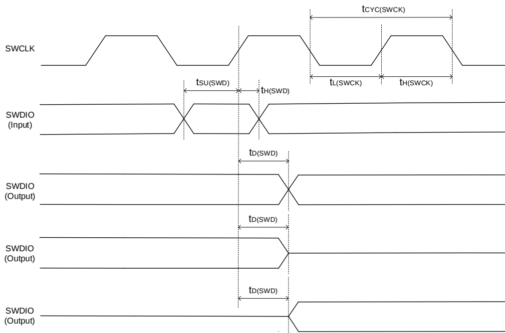
Figure 4-18. SWD timing diagram
