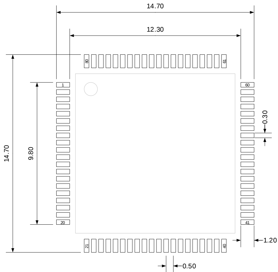
Figure 5-8. LQFP80 recommended footprint
