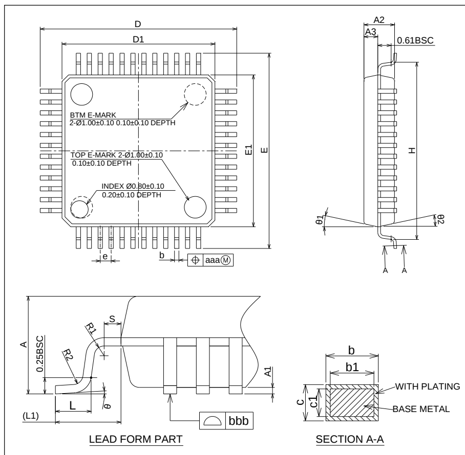
Figure 5-11. LQFP48 package outline
