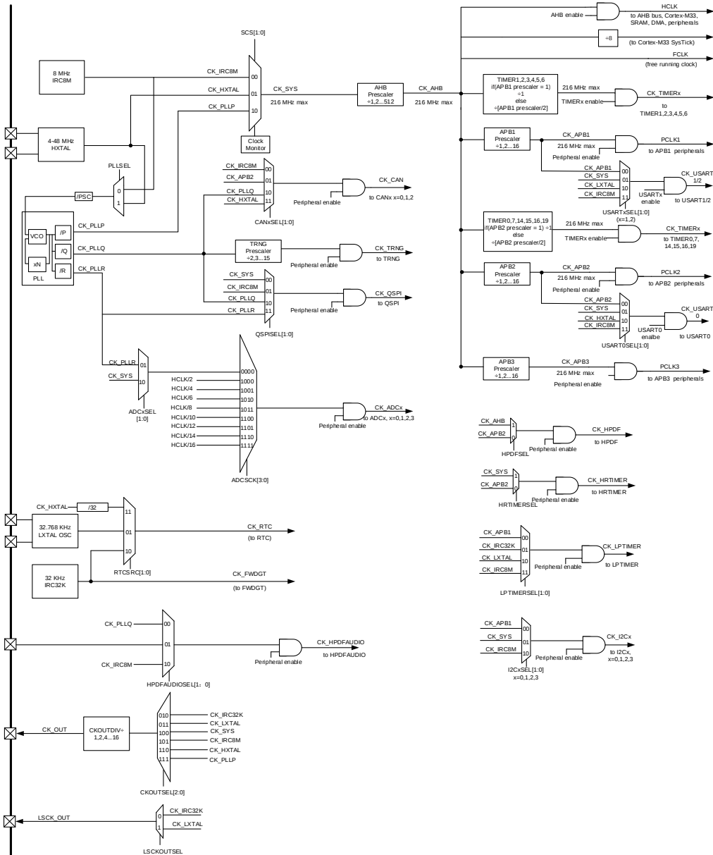
Figure 2-9. GD32G553xx clock tree
