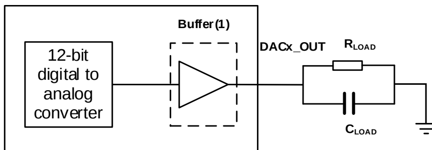
Figure 4-10. 12-bit buffered /non-buffered DAC
