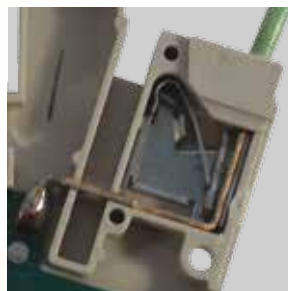
Push-in terminal
