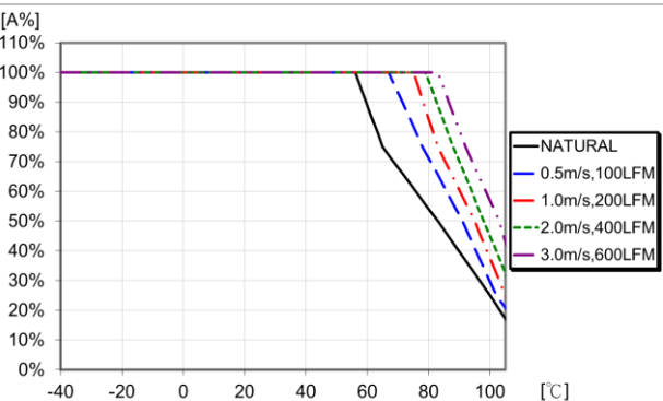
Available load current vs. ambient air temperature and airflow at V_1 = 36 V with 20 mm half brick heat sink. See Thermal Consideration section.
