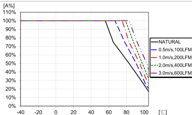
Available load current vs. ambient air temperature and airflow at V_1 = 36 V with 12.7 mm half brick heat sink. See Thermal Consideration section.
