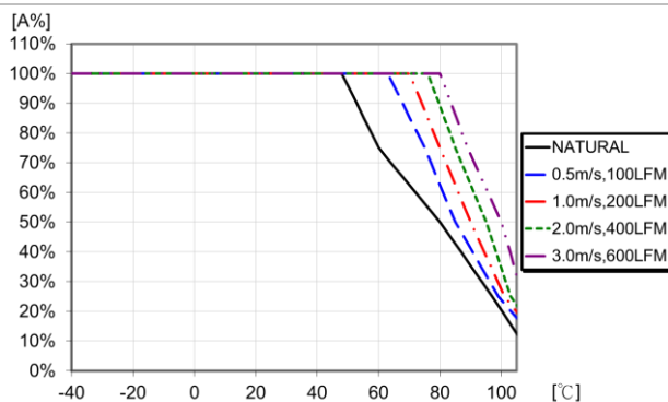
Available load current vs. ambient air temperature and airflow at V_1 = 36 V. See Thermal Consideration section.
