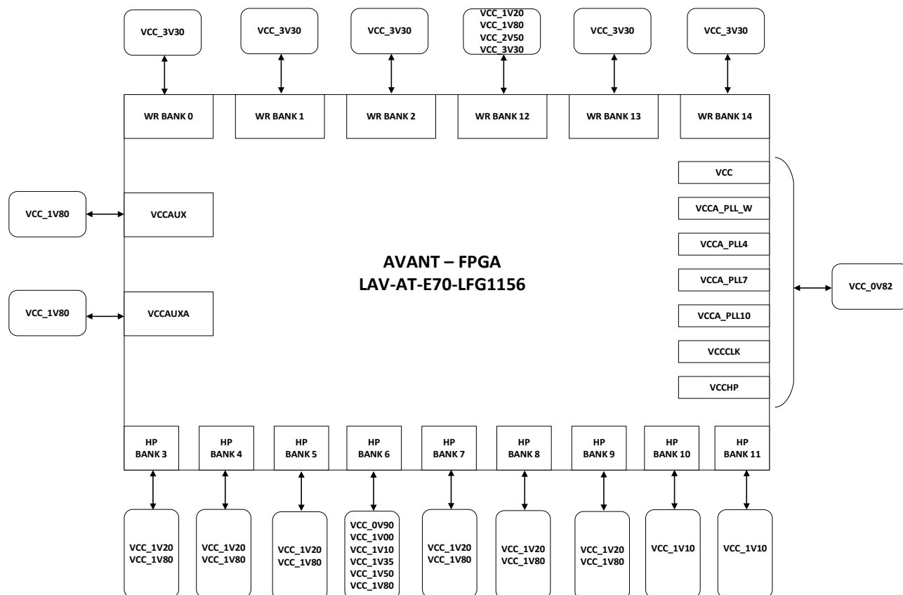
Figure 3.2. Board Power Scheme (2)
