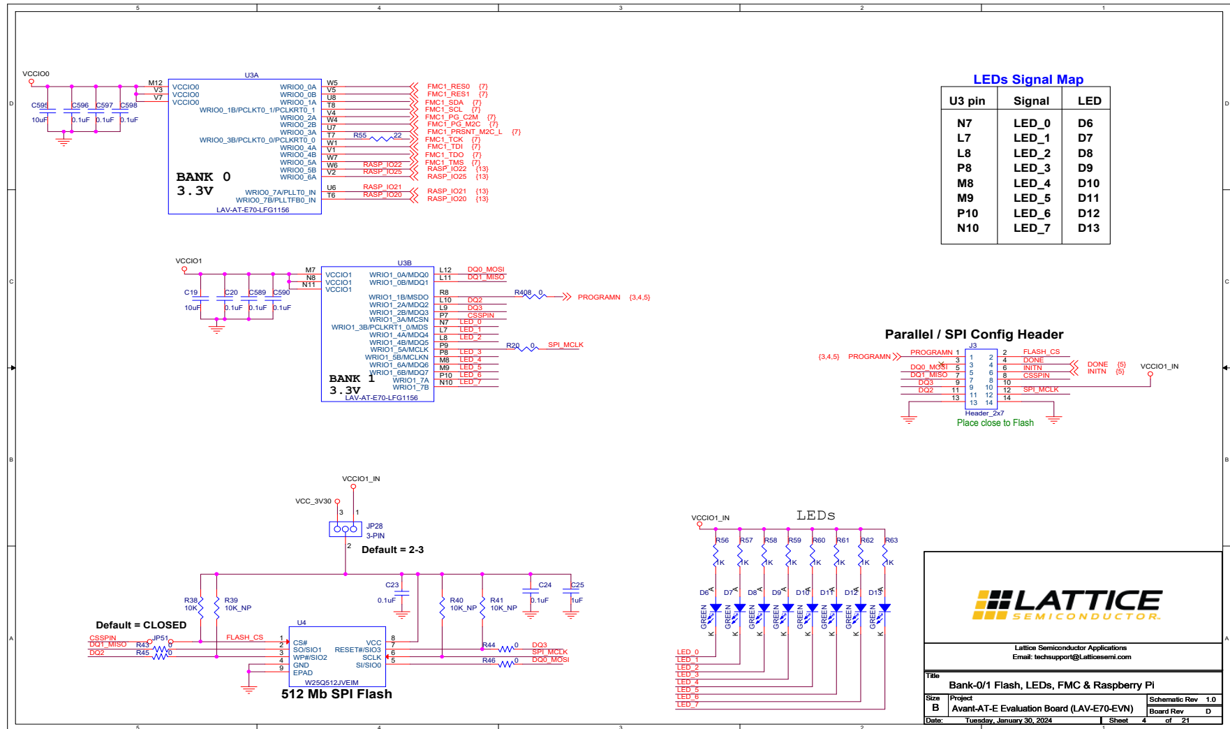
Figure A.4. Bank-0/1 Flash, LEDs, FMC & Raspberry Pi
