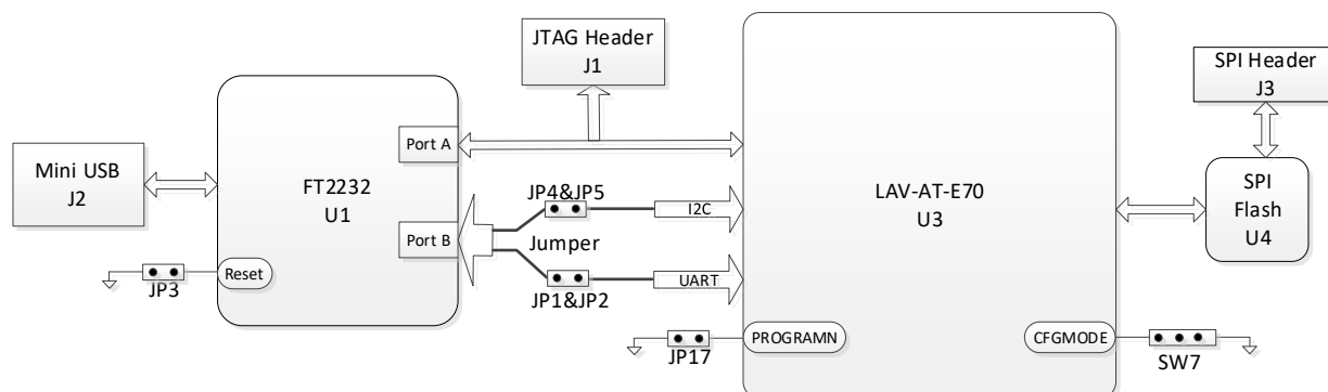
Figure 5.1. Configuration, UART and I²C Architecture
