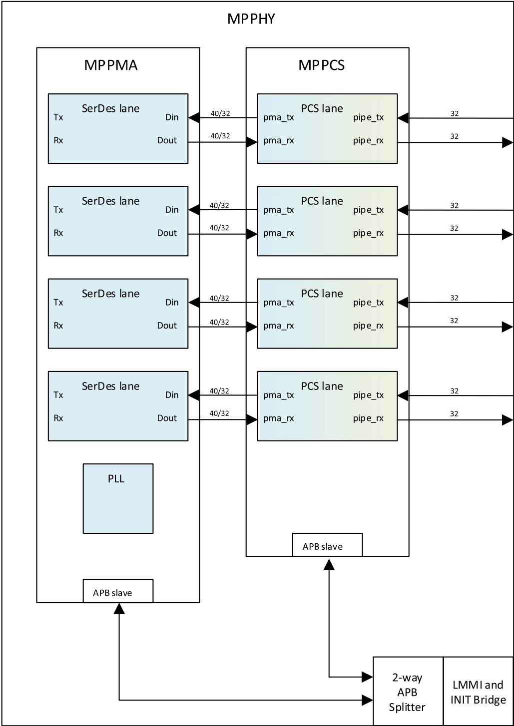
Figure 2.15. MPPHY Top-Level Block Diagram
