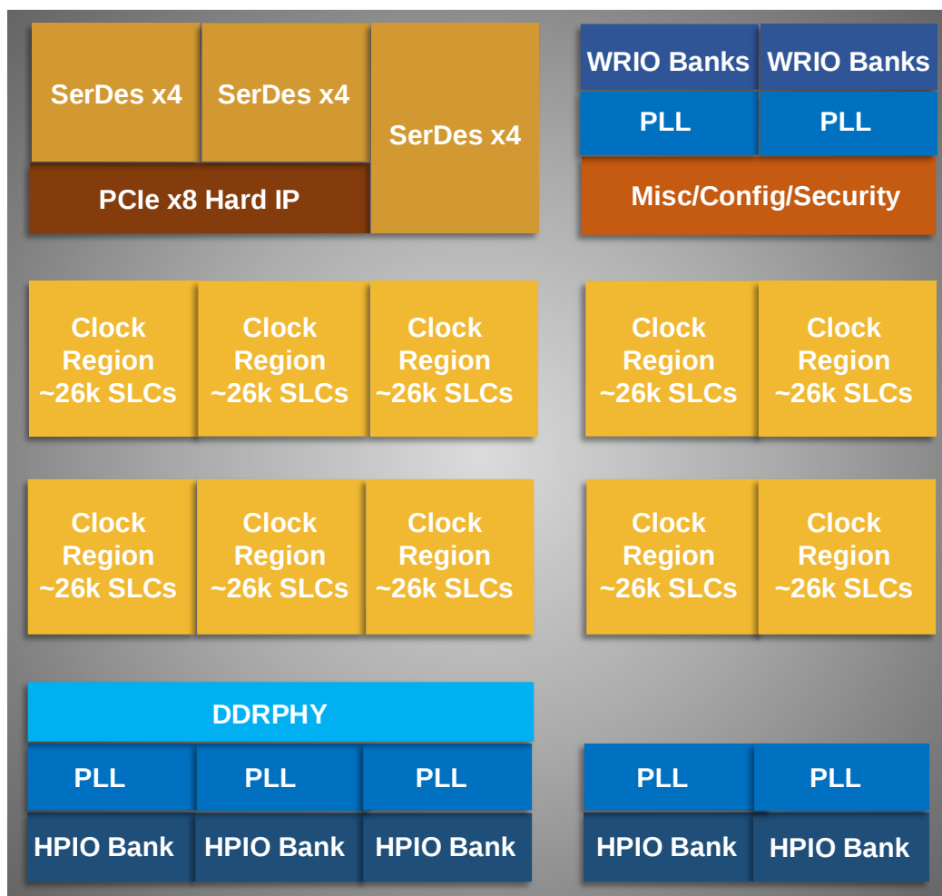
Figure 2.1. High-level Device Floorplan (LAV-AT-E/G/X30 Device)
