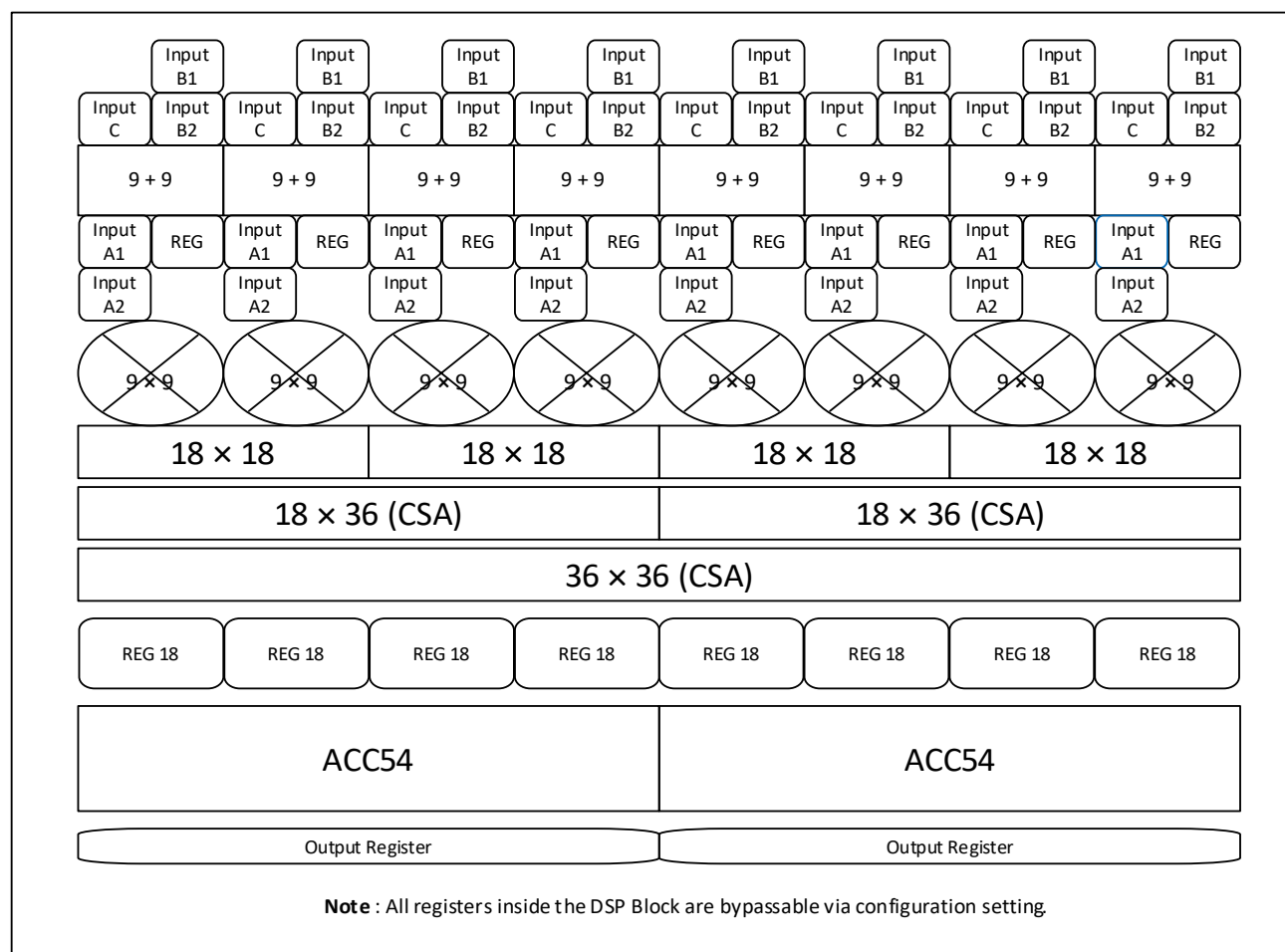
Figure 2.16. CertusPro-NX DSP Functional Block Diagram
