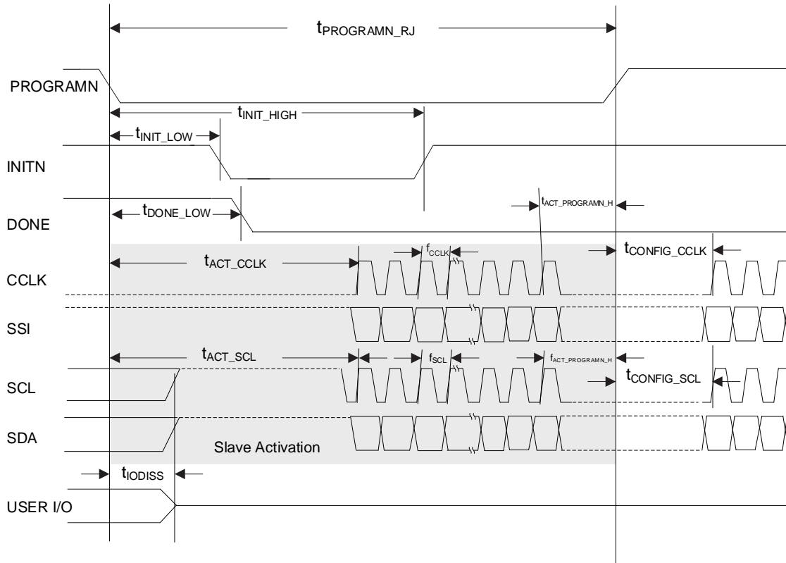
Figure 4.17. Slave SPI/I²C/I³C PROGRAMN Timing
