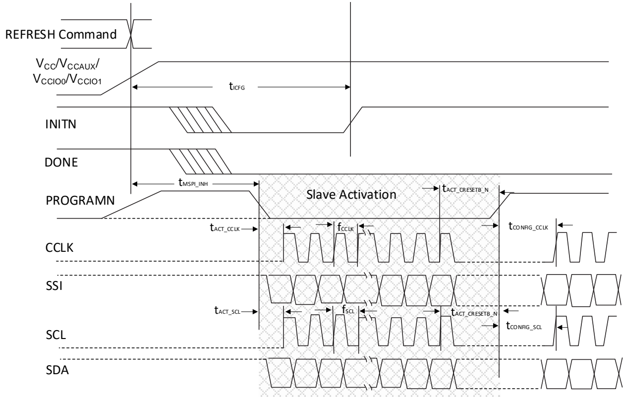
Figure 4.15. Slave SPI/I²C/I³C POR/REFRESH Timing
