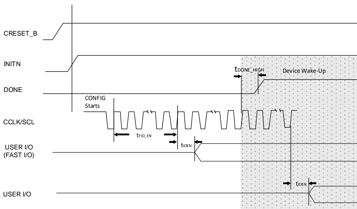
Figure 4.22. Slave SPI/I²C/I³C Wake-Up Timing
