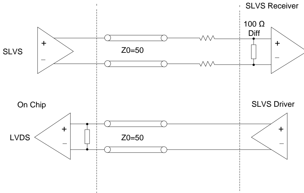
Figure 3.5. SLVS Interface
