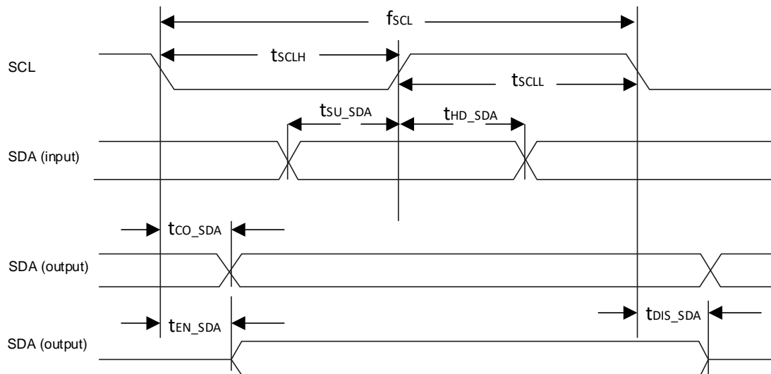
Figure 4.20. I²C/I3C Configuration Timing
