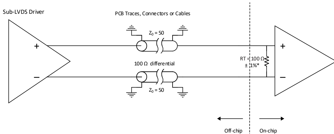
Figure 4.3. SubLVDS Input Interface
