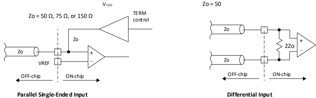
Figure 3.1. On-chip Termination
