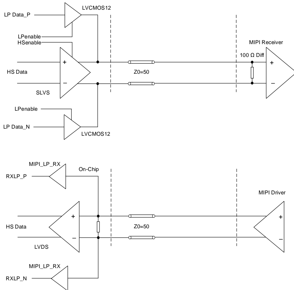
Figure 3.6. MIPI Interface
