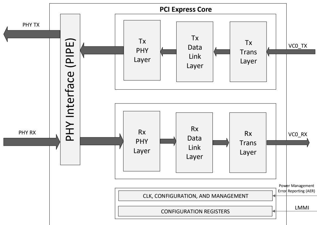
Figure 2.34. PCIe Core
