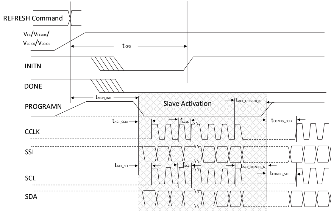
Figure 3.15. Slave SPI/I²C/I³C POR/REFRESH Timing
