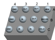
WLCSP-12 CASE 567WP
