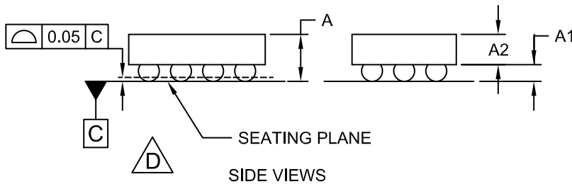
SIDE VIEWS
