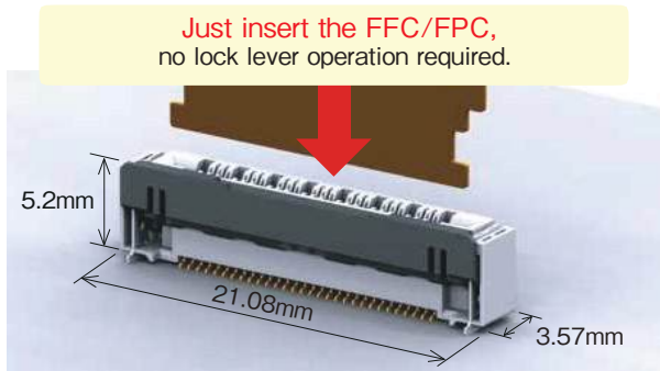
One Action Lock (Dimensions Shown : 30pos.)
