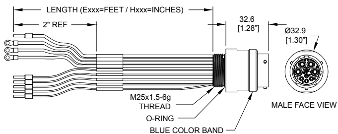
FIG 4: Male, Receptacle, Straight, 9 Position
