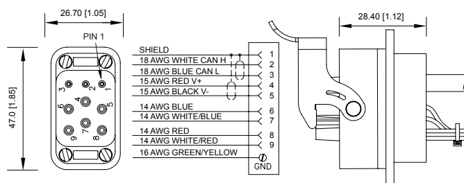
FIG 6: Female Power, Receptacle, Straight, 9 Position
