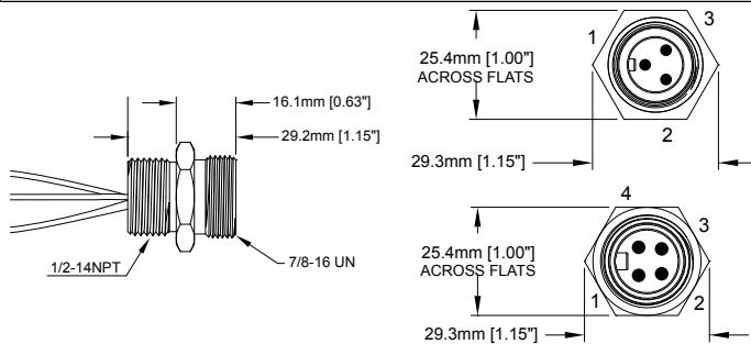
FIG 5: Male, Receptacle, Straight, Drop, 3 and 4 Position
