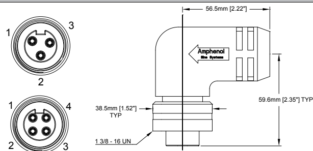
FIG 4: Female, Plug, 90°, Trunk, 3 and 4 Position
