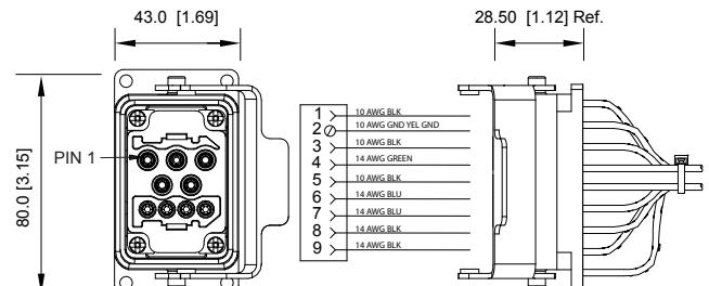
FIG 6: Female Power, Straight, Receptacle
