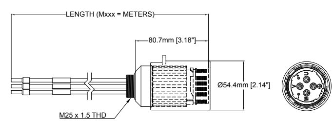
FIG 6: Male, 10AWG, Receptacle w/ M25 Threaded Adapter
