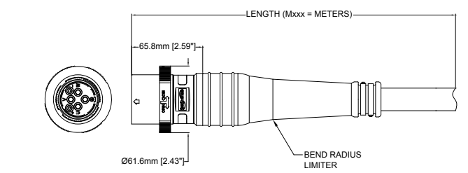
FIG 3: Male to Female, Plug, Straight, 6 Position
