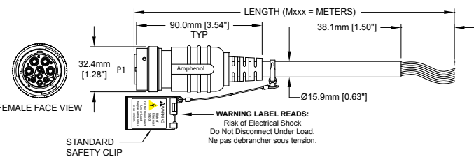
FIG 2: Female, Plug, Straight, 9 Position
