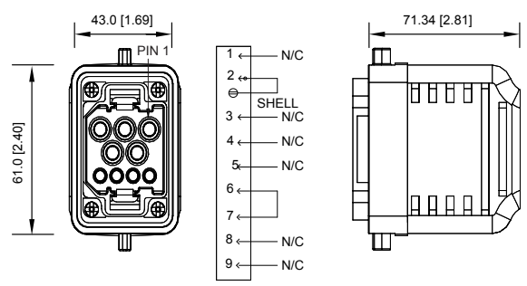
FIG 10: Male, Single Channel, Terminator, 9 Position
