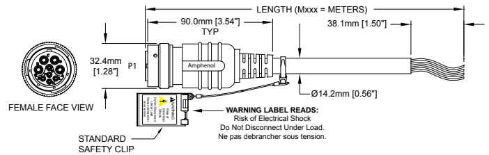
FIG 2: Female, Plug, Straight, 9 Position
