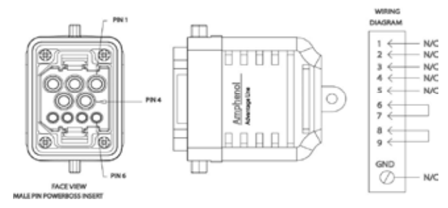
FIG 11: Male, Dual Channel, Terminator, 9 Position
