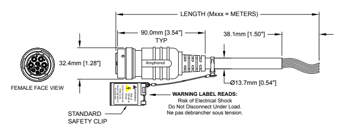
FIG 2: Female, Plug, Straight, 9 Position
