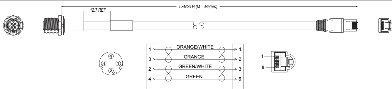
FIG 6: P29930-Mxxx, Ethernet M12, Female Receptacle to RJ45, Blue
