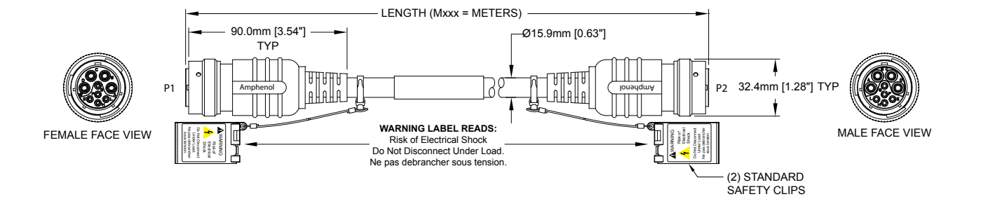
FIG 3: Male Plug to Female Plug, Straight, 9 Position
