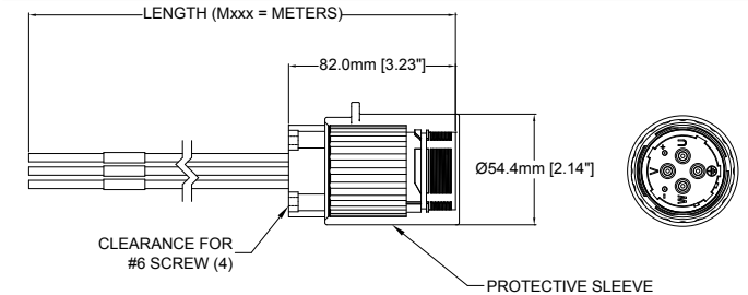
FIG 6: Male, 10AWG, Receptacle w/ M25 Threaded Adapter
