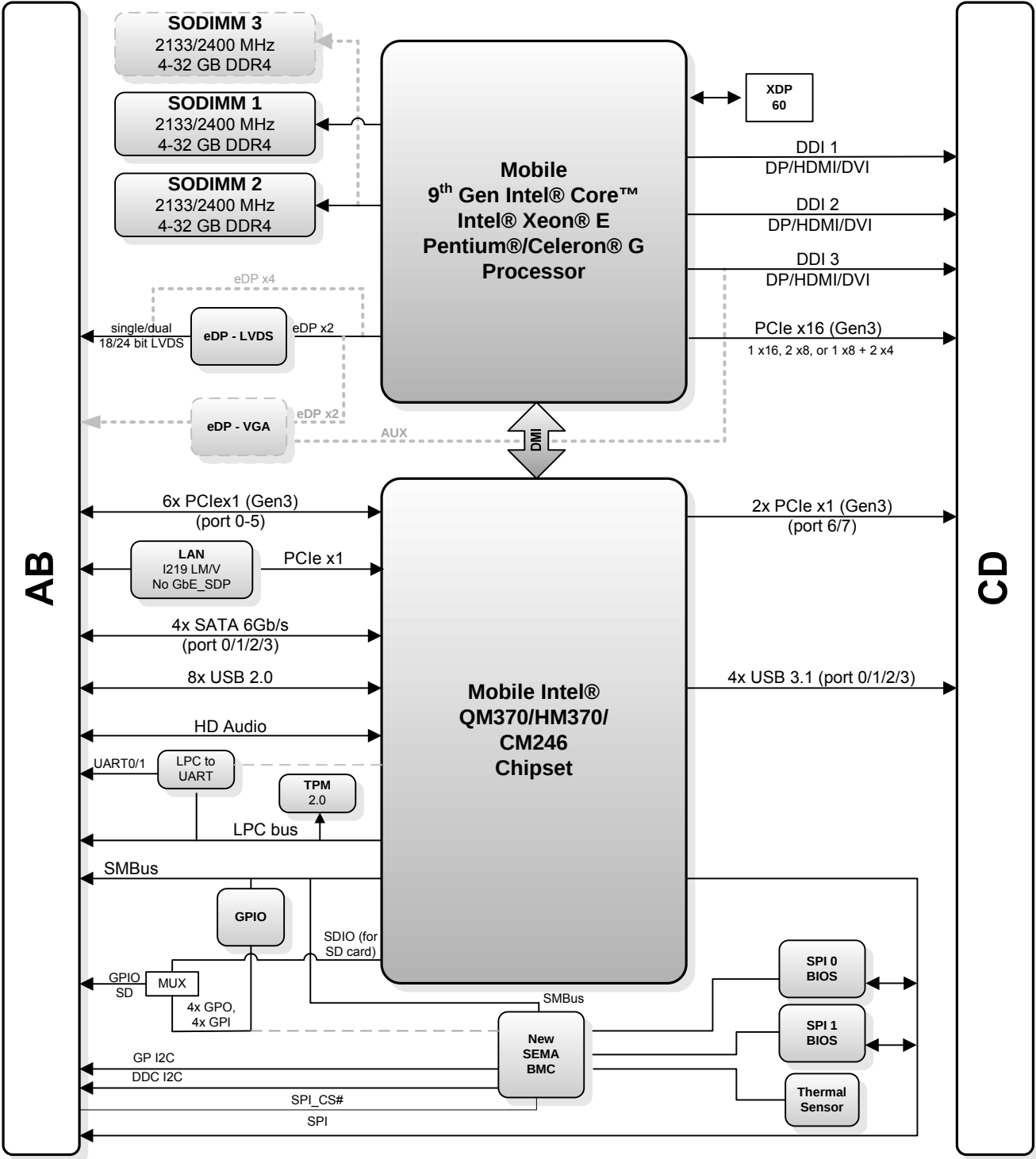
Figure 1: Express-CFR Functional Block Diagram
