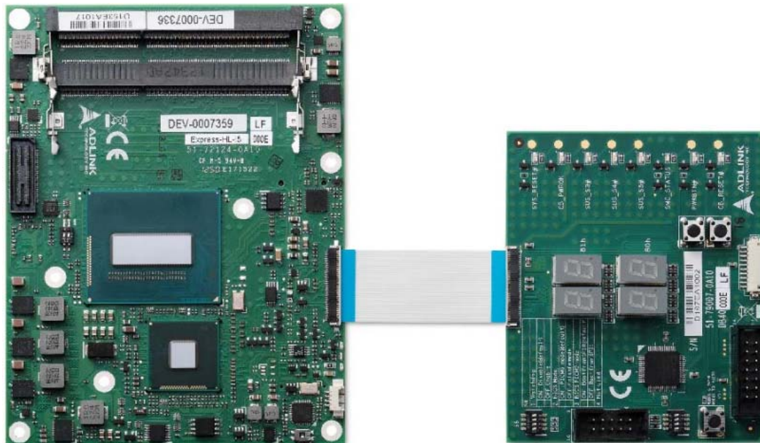
Figure 4: Express-CFR and the DB40 Debug Module
