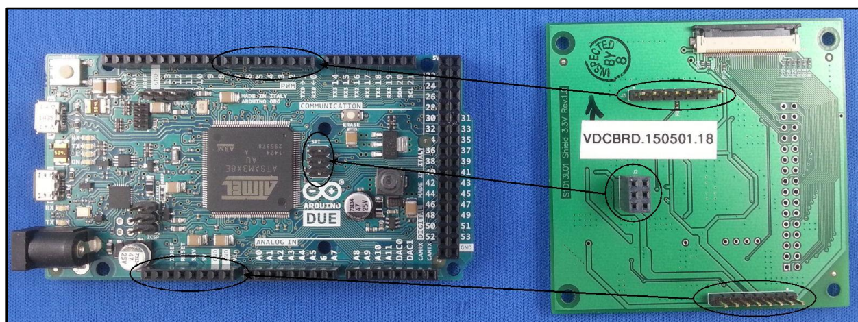
S1D13781 Shield to Arduino Due Connections
