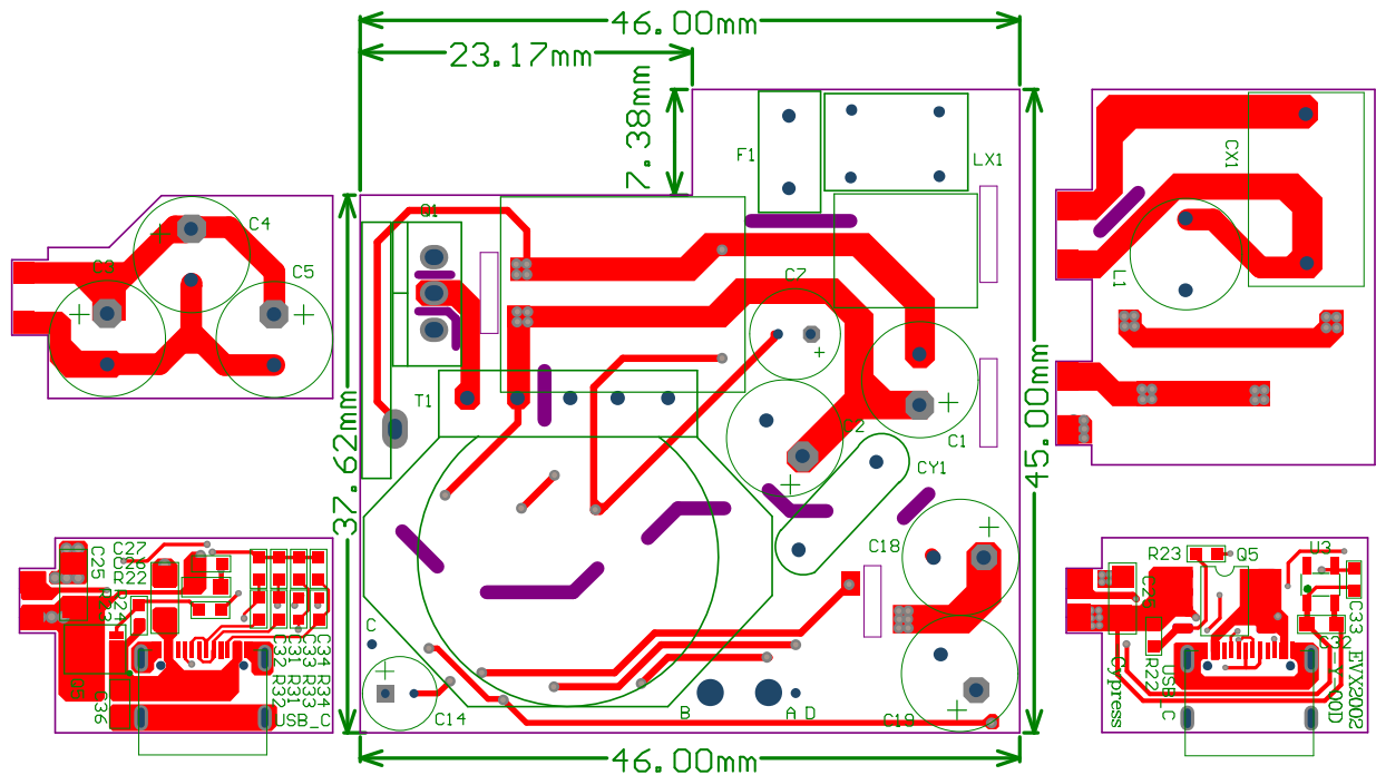
Figure 4: Top Layer
