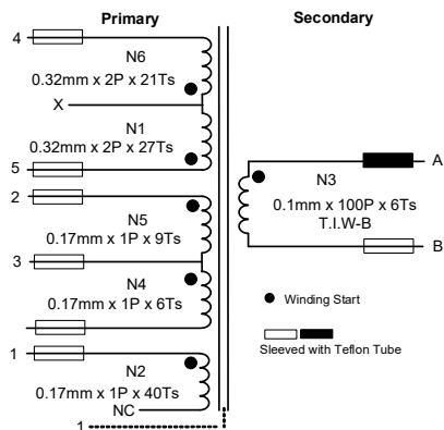
Figure 6: Electrical Diagram
