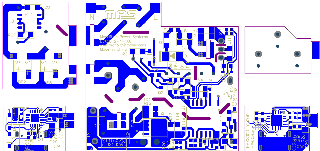
Figure 5: Bottom Layer
