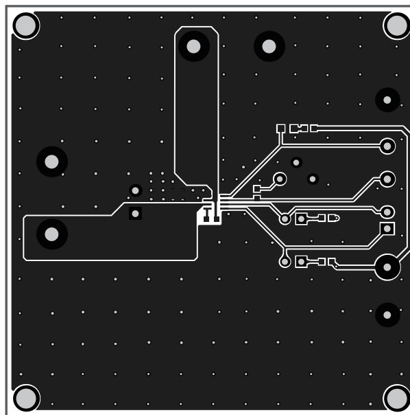
Figure 3: Top Layer
