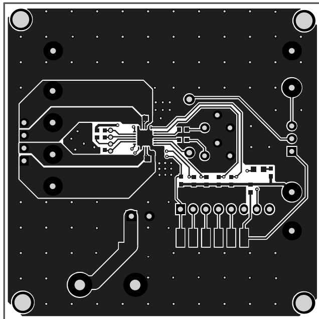
Figure 3: Top Layer
