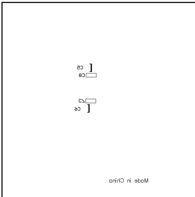
Figure 5: Bottom Silk
