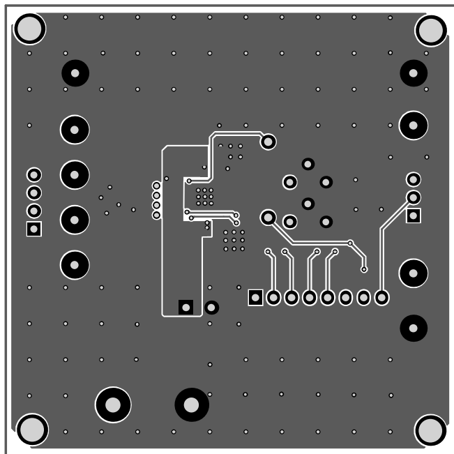
Figure 4: Bottom Layer
